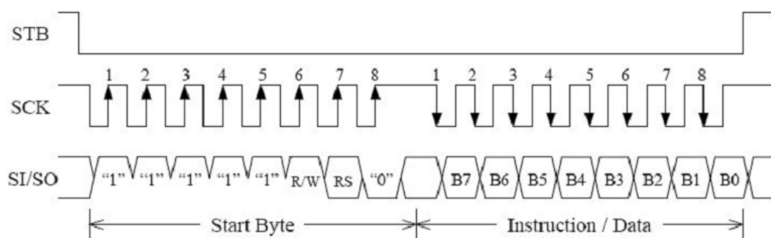
Typical Synchronous Serial Interface Read Cycle
