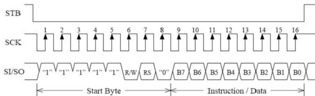
Typical Synchronous Serial Interface Write Cycle
