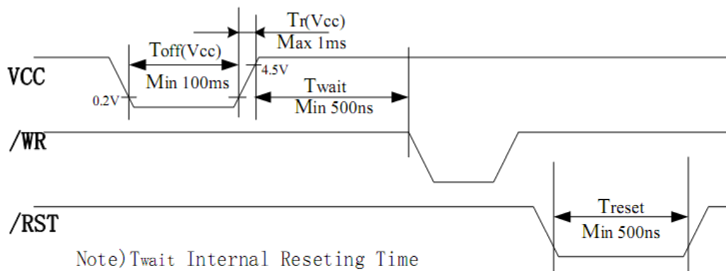
Fig-1 Power-on Reset and RESET signal Timing
