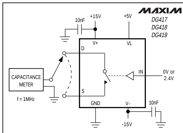
Figure 9. Drain-Source On-Capacitance
