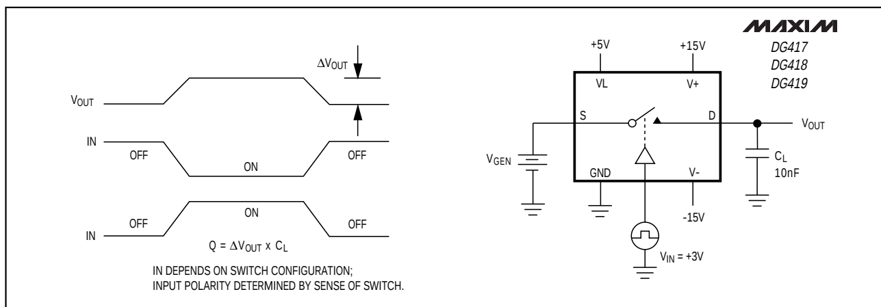
Figure 5. Charge Injection
