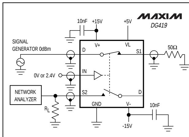
Figure 7. DG419 Crosstalk
