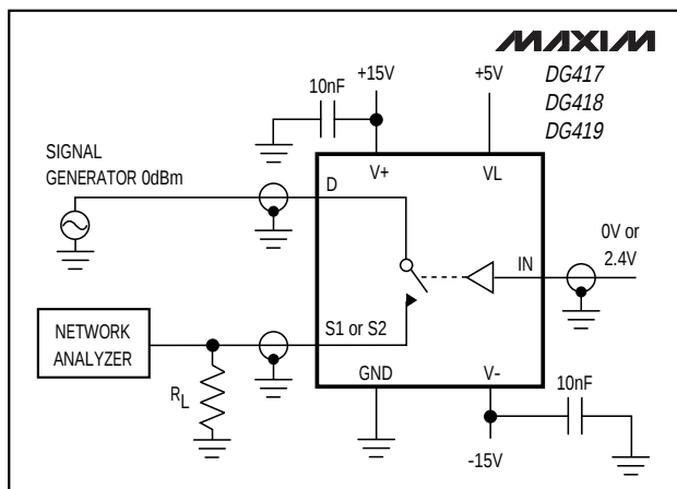
Figure 6. Off-Isolation Rejection Ratio
