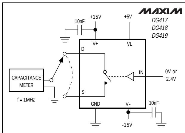
Figure 8. Drain-Source Off-Capacitance
