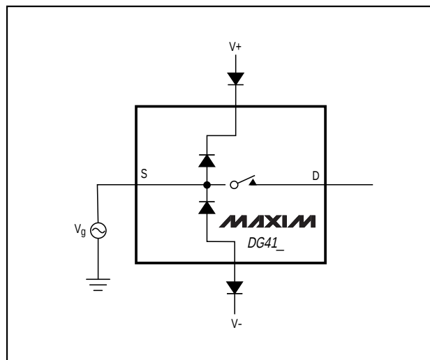
Figure 1. Overvoltage Protection Using External Blocking Diodes
