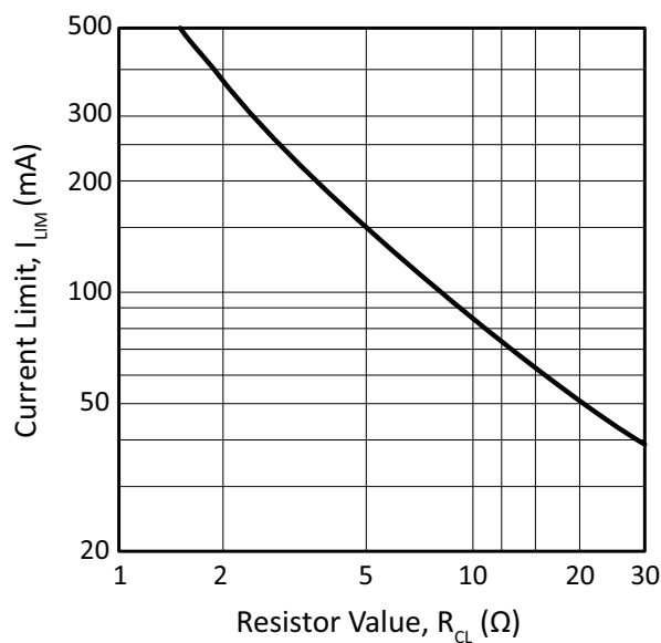
Figure 14: Current Limit
