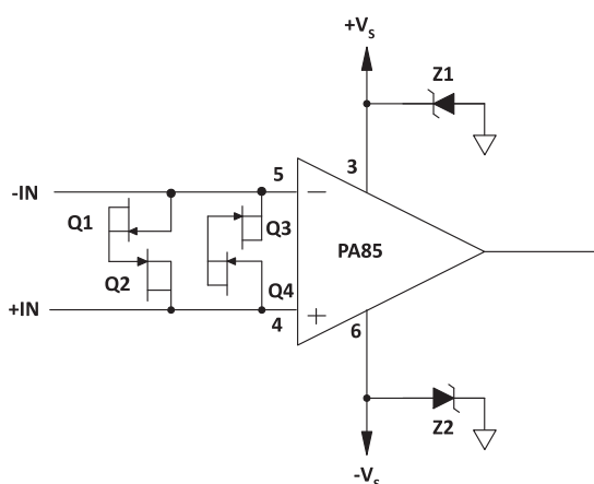
Figure 17: Overvoltage Protection
