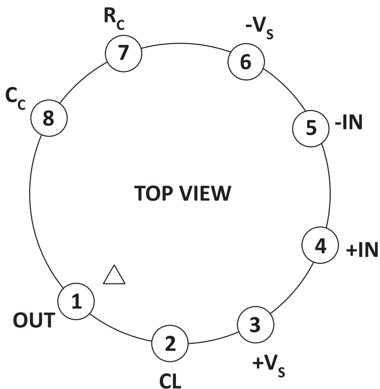
Figure 2: External Connections
