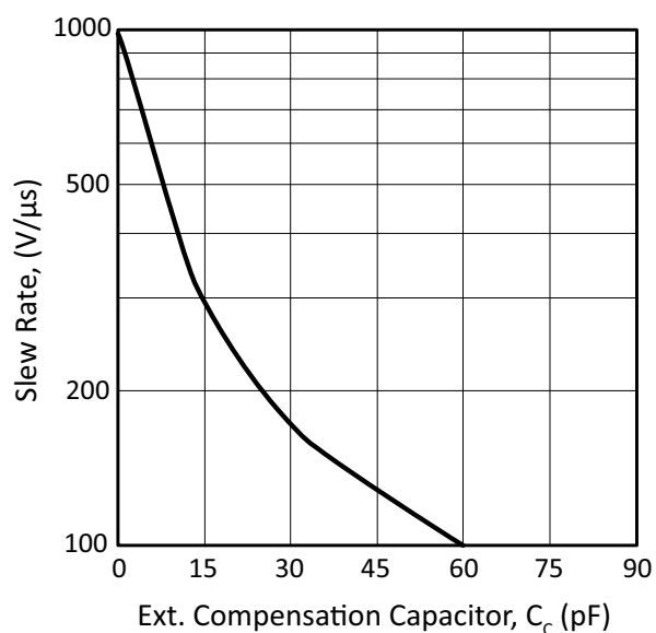
Figure 9: Slew Rate
