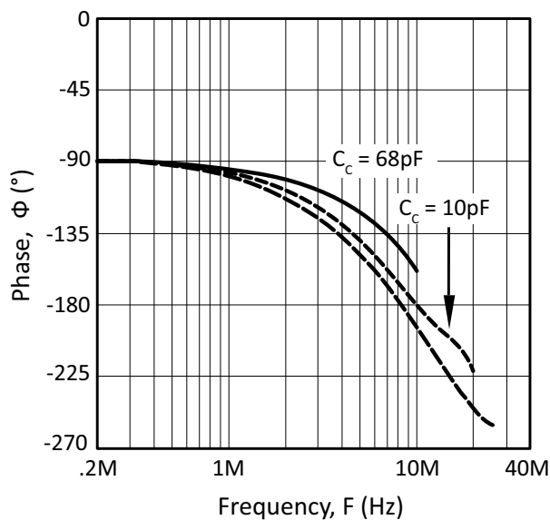
Figure 6: Phase Response
