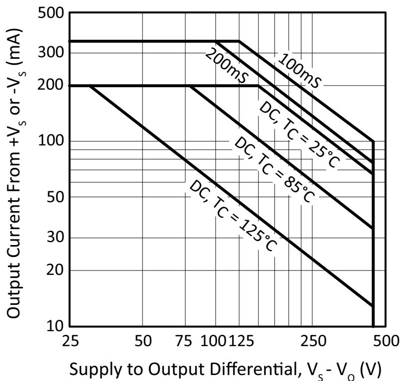
Figure 15: SOA
