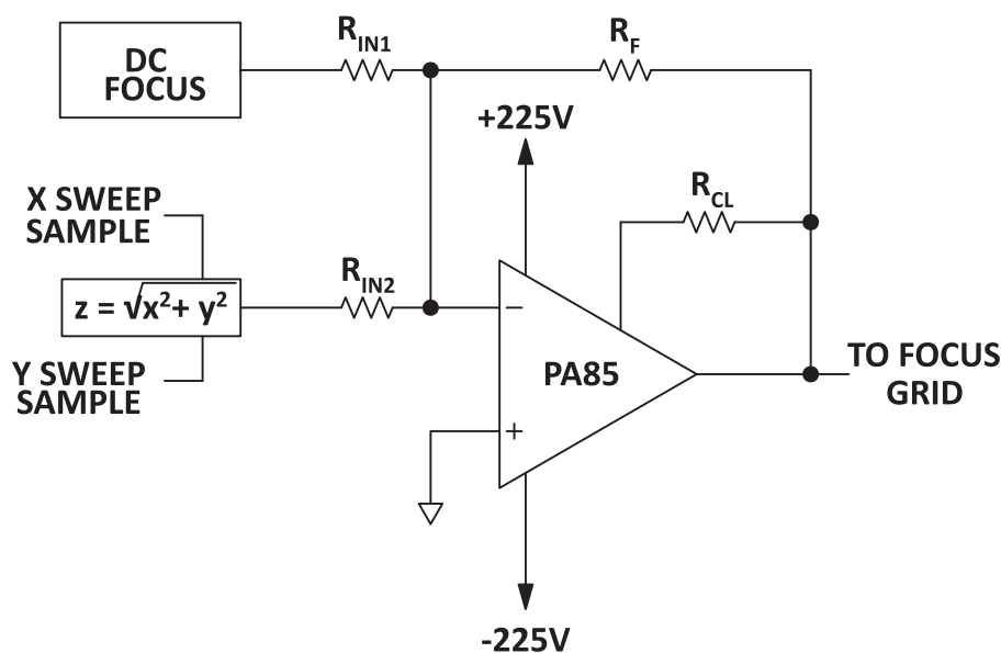
Figure 16: Typical Application
