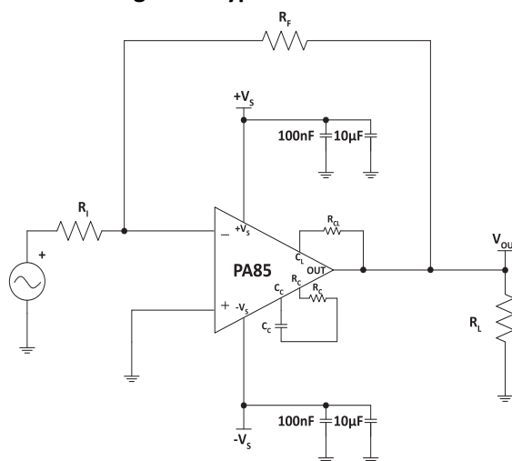
Figure 1: Typical Connection
