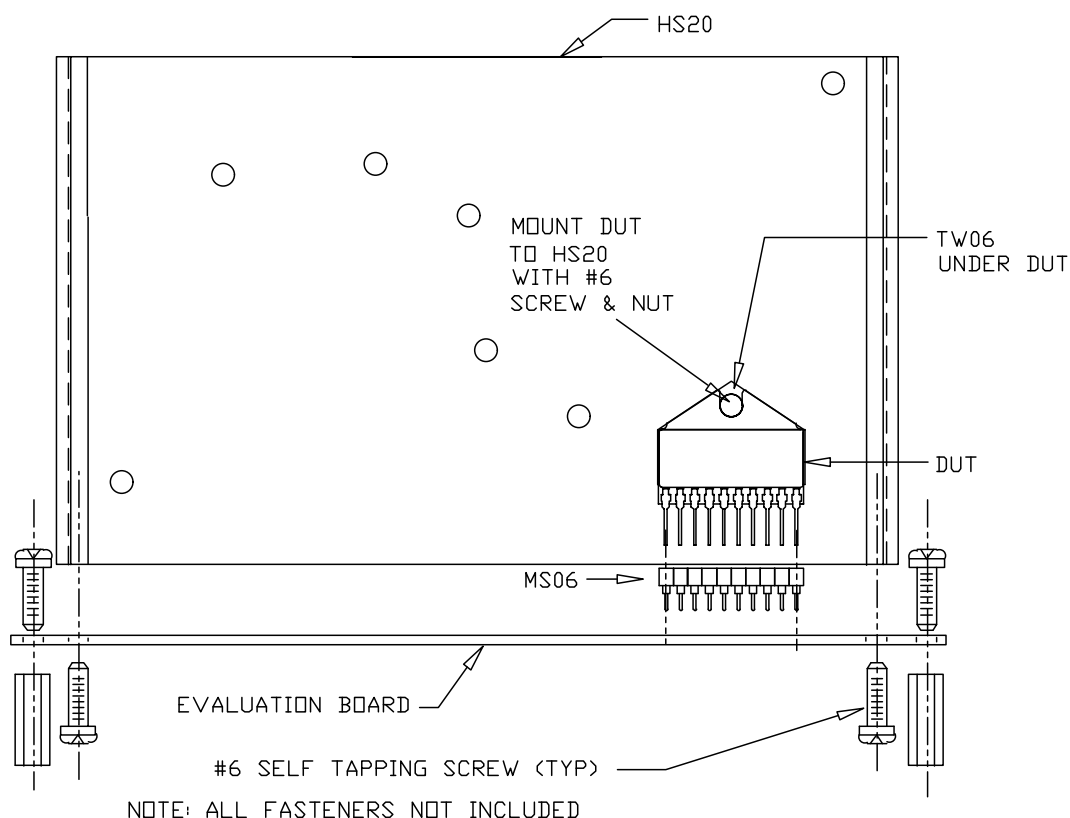
Figure 1: Assembly Diagram for EK06
