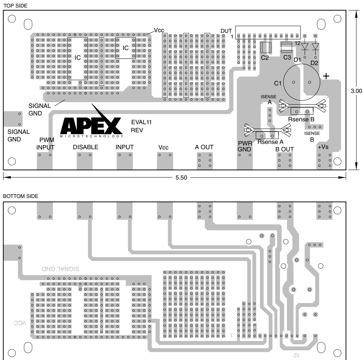
Figure 2: PCB Board
