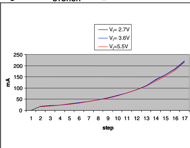
Figure 18. I_{O\text{AUX}} vs. AUX1
