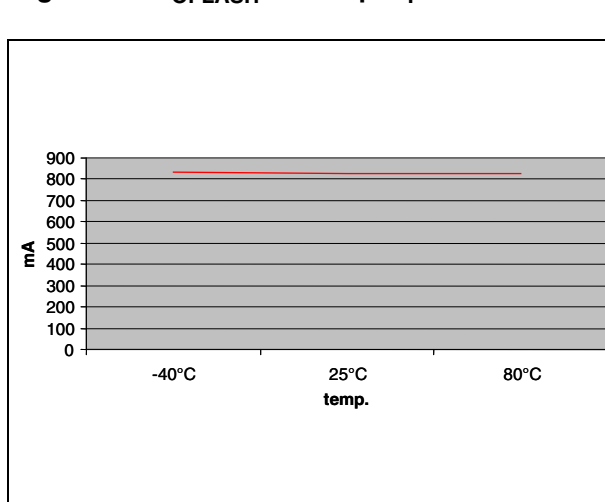
Figure 19. I_{O\text{FLASH}} vs. temp. V_i = 3.3\text{V}
