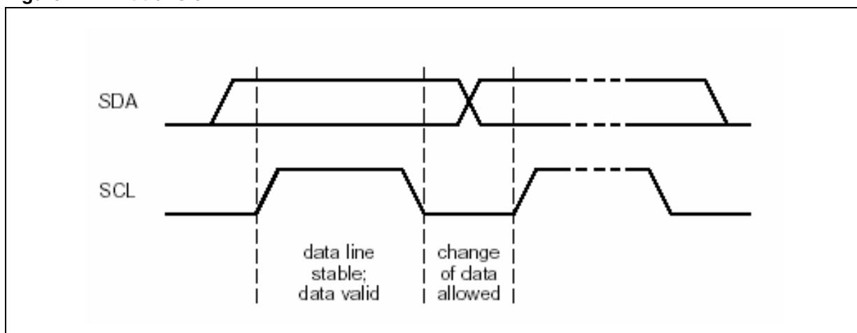
Figure 7. Bit transfer
