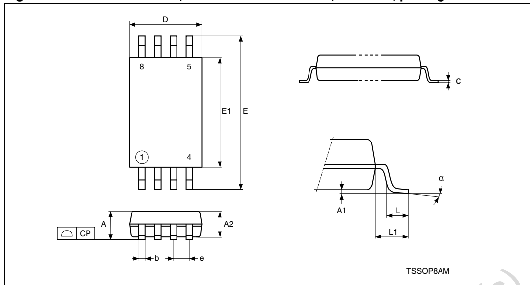
Figure 8. TSSOP8 – 8-lead, thin shrink small outline, 3x4.4mm, package outline
