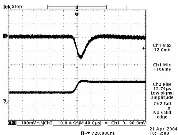
50% to 100% load Transient at Vin=12 V, Vo=1.2 V
