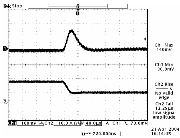
100% to 50% load Transient at Vin=5 V, Vo=1.5 V
