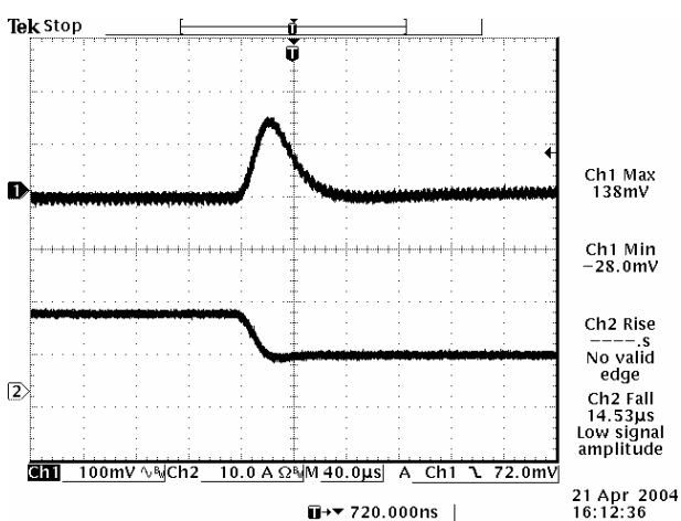
100% to 50% load Transient at Vin=5 V, Vo=1.2 V
