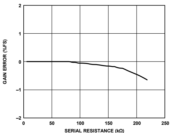
Figure 12. Capacitance Input Gain Error vs. Serial Resistance V_{DD} = 3.3 V, CIN to EXC = 2 pF
