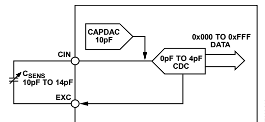
Figure 22. Using CAPDAC
