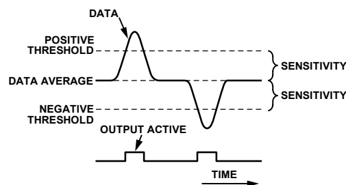
Figure 35. Threshold Sensitivity
