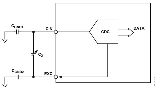
Figure 42. Parasitic Capacitance to Ground
