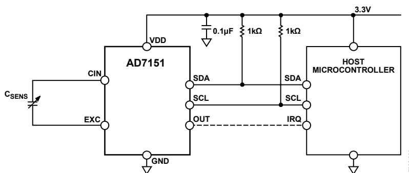
Figure 50. AD7151 Interfaced to a Host Microcontroller
