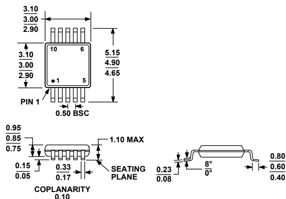
Figure 52. 10-Lead Mini Small Outline Package [MSOP] (RM-10)
