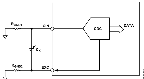
Figure 43. Parasitic Resistance to Ground
