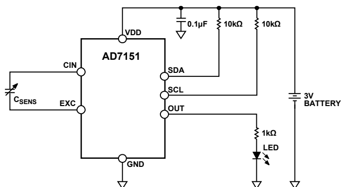
Figure 49. AD7151 Standalone Operation Application Diagram
