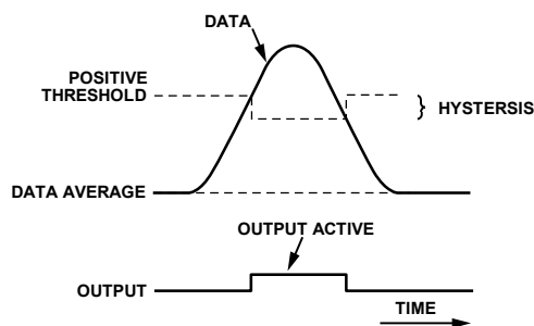
Figure 30. Threshold Hysteresis
