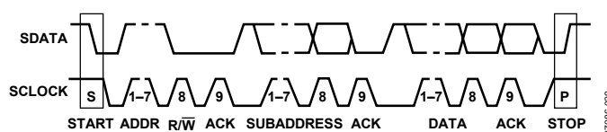
Figure 40. Bus Data Transfer
