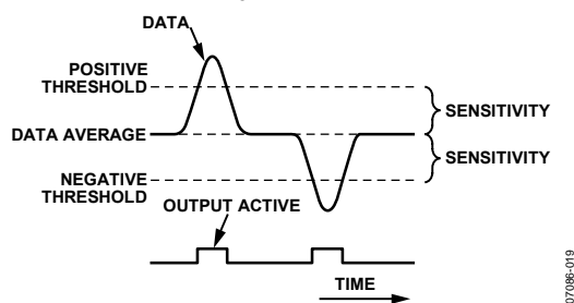
Figure 29. Threshold Sensitivity
