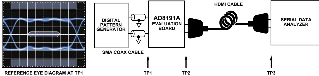
Figure 9. Test Circuit Diagram for Tx Eye Diagrams
