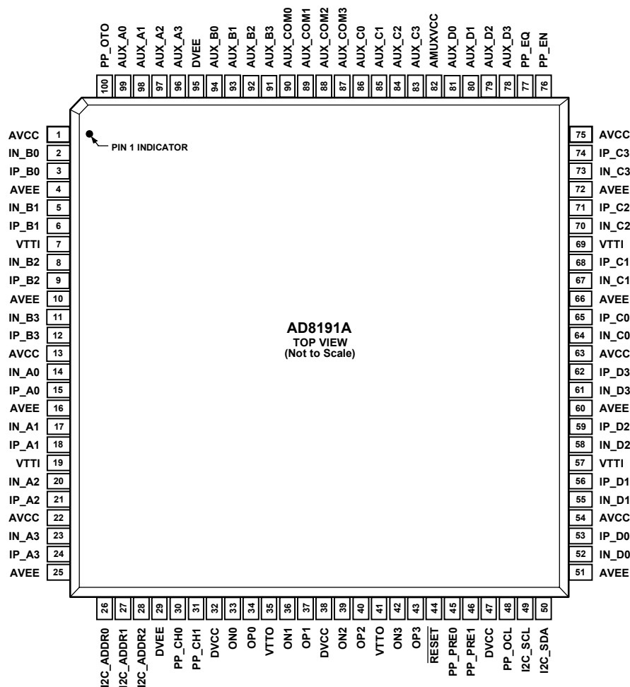
Figure 3. Pin Configuration
