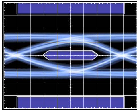
0.125UI/DIV AT 1.65Gbps
