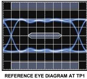
REFERENCE EYE DIAGRAM AT TP1
