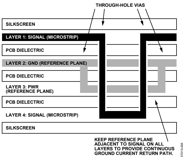
Figure 32. Example Routing of Reference Plane
