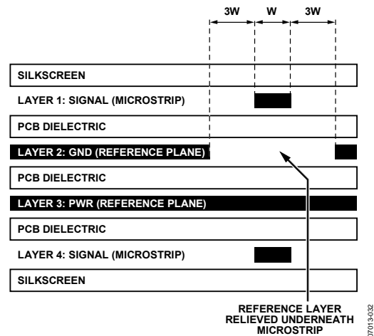
Figure 33. Example Board Stackup
