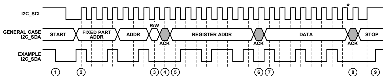
*THE SWITCHING/UPDATE DELAY BEGINS AT THE FALLING EDGE OF THE LAST DATA BIT; FOR EXAMPLE, THE FALLING EDGE JUST BEFORE STEP 8.
