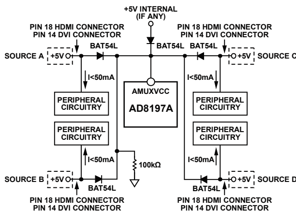
Figure 28. Suggested AMUXVCC Power Scheme
