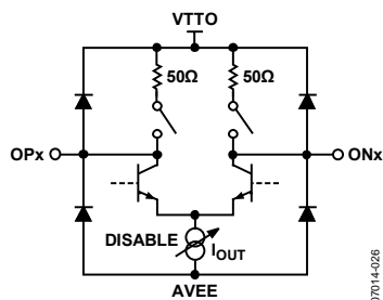
Figure 26. High Speed Output Simplified Schematic
