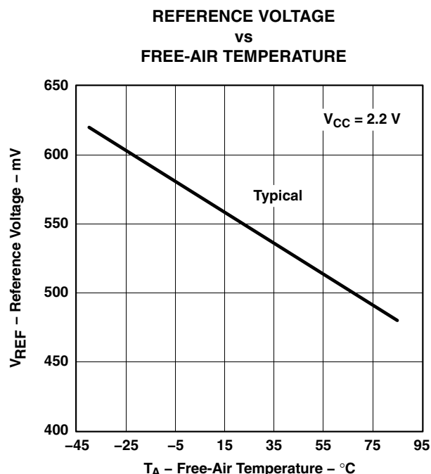
Figure 18. V (RefVT) vs Temperature
