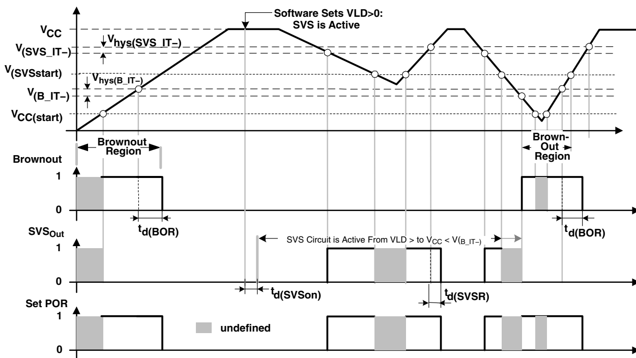
Figure 11. SVS Reset (SVSR) vs Supply Voltage
