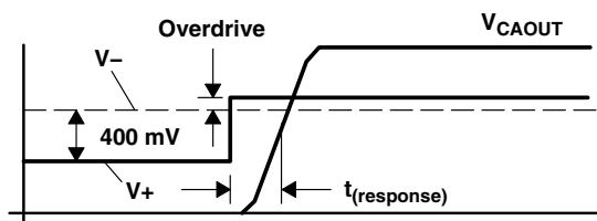
Figure 20. Overdrive Definition
