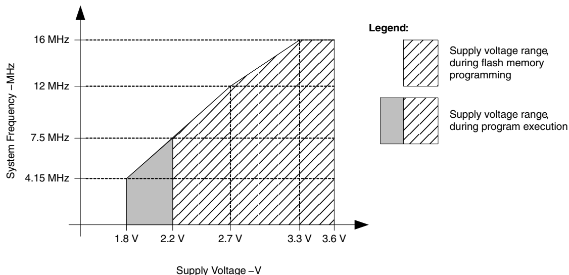
Figure 1. Operating Area
