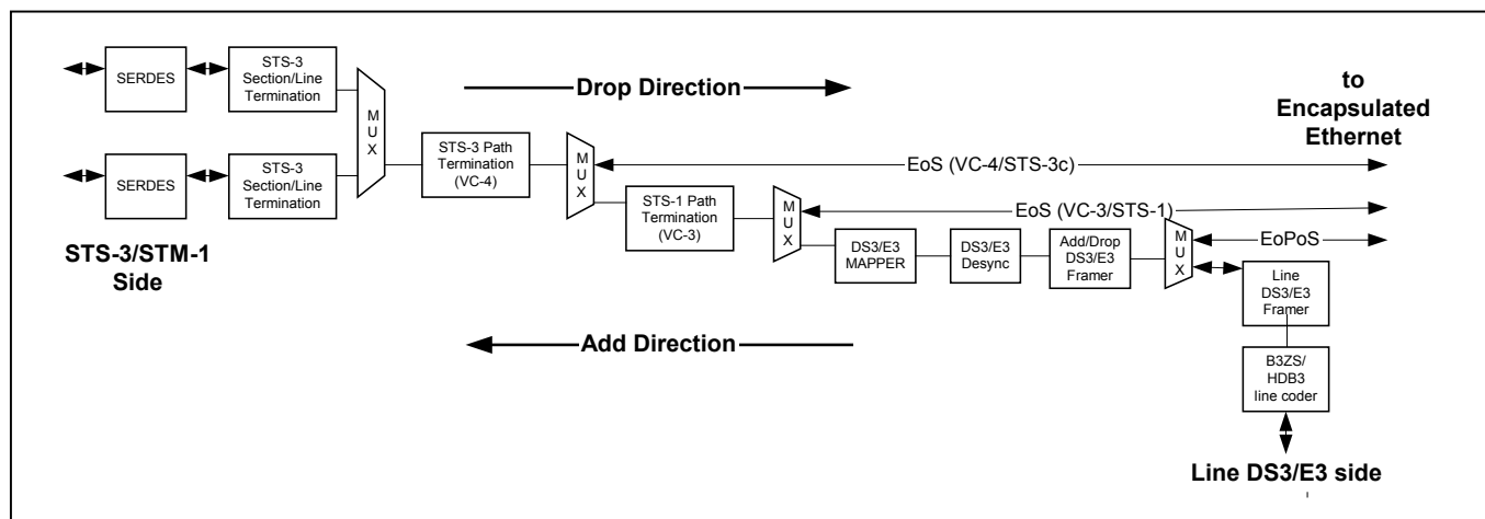
Figure 1-1. TDM Functional Blocks
