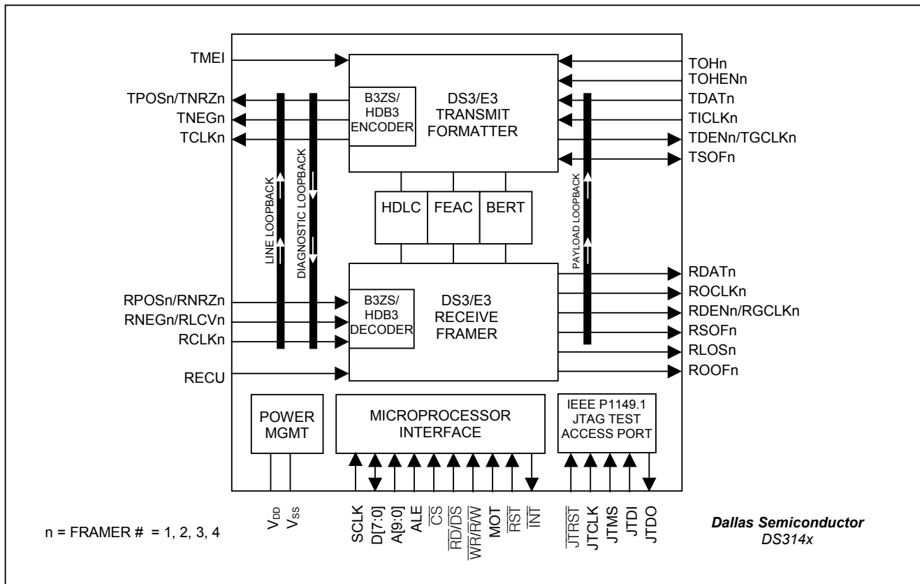
Figure 1-1. Block Diagram
