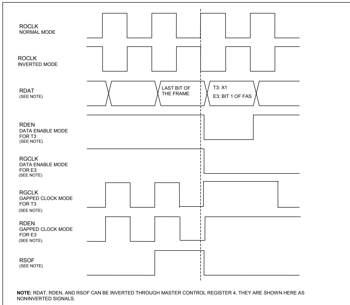
Figure 5-2. Receive Framer Timing
