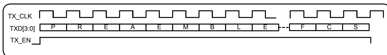
Figure 11-20. MII Transmit Functional Timing
