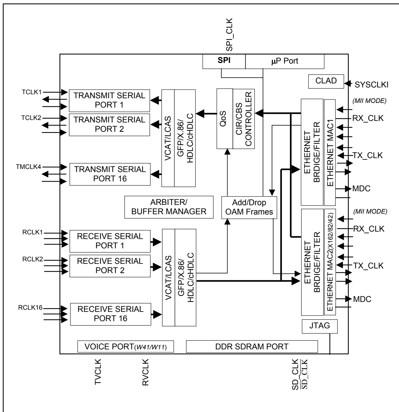
Figure 8-1. Clocking Diagram
