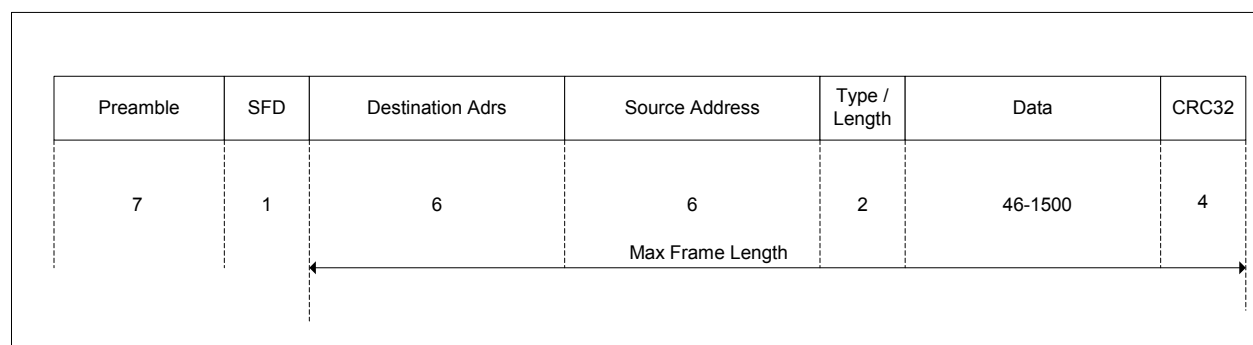
Figure 8-8. IEEE 802.3 Ethernet Frame
