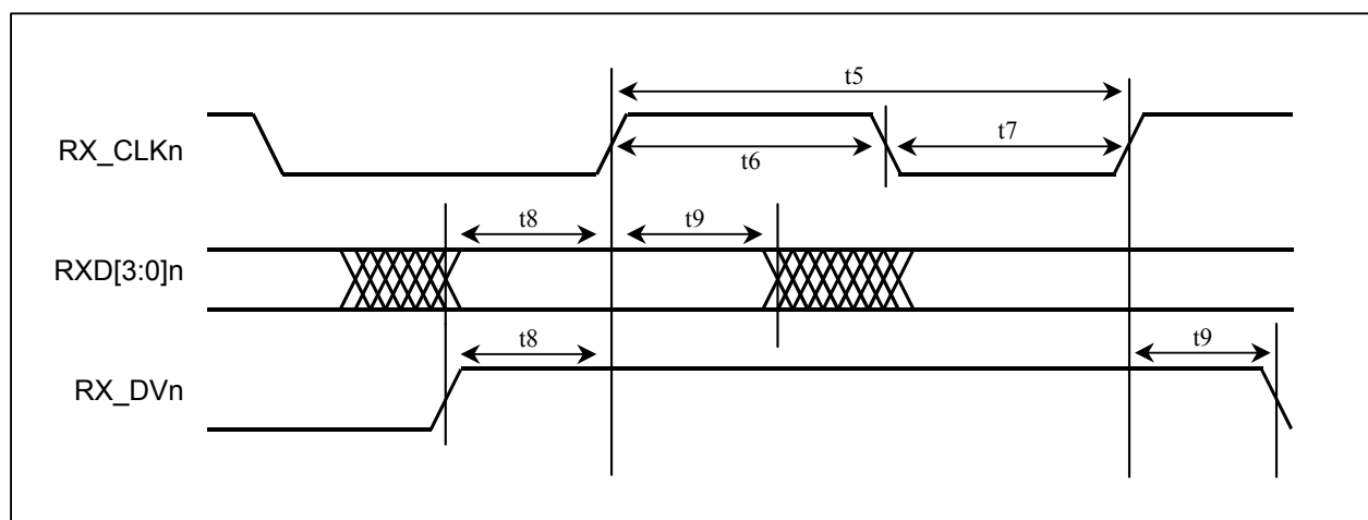
Figure 12-4. Receive MII Interface Timing
