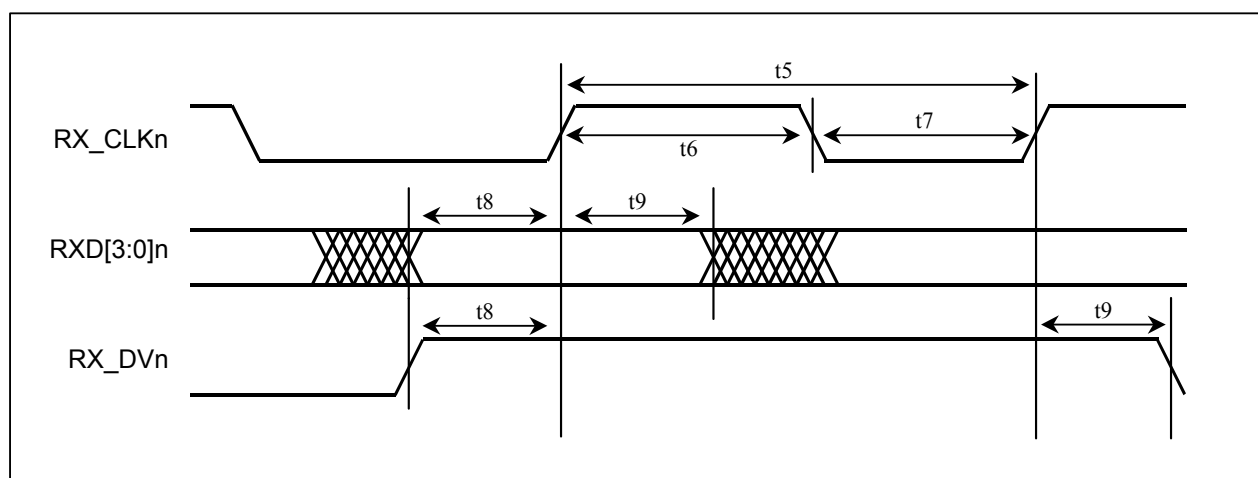
Figure 12-2. Receive GMII Interface Timing
