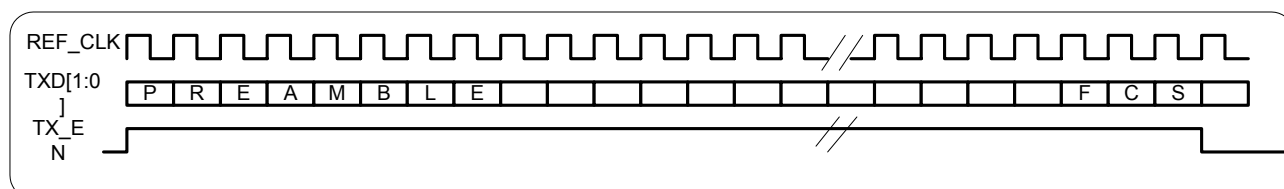
Figure 11-18. GMII Transmit Interface Functional Timing
