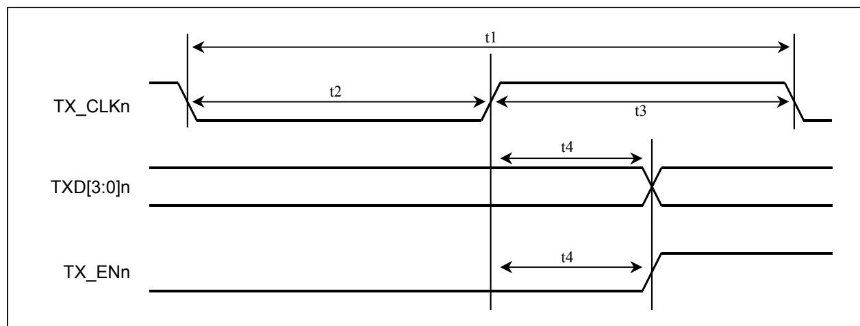
Figure 12-3. Transmit MII Interface Timing
