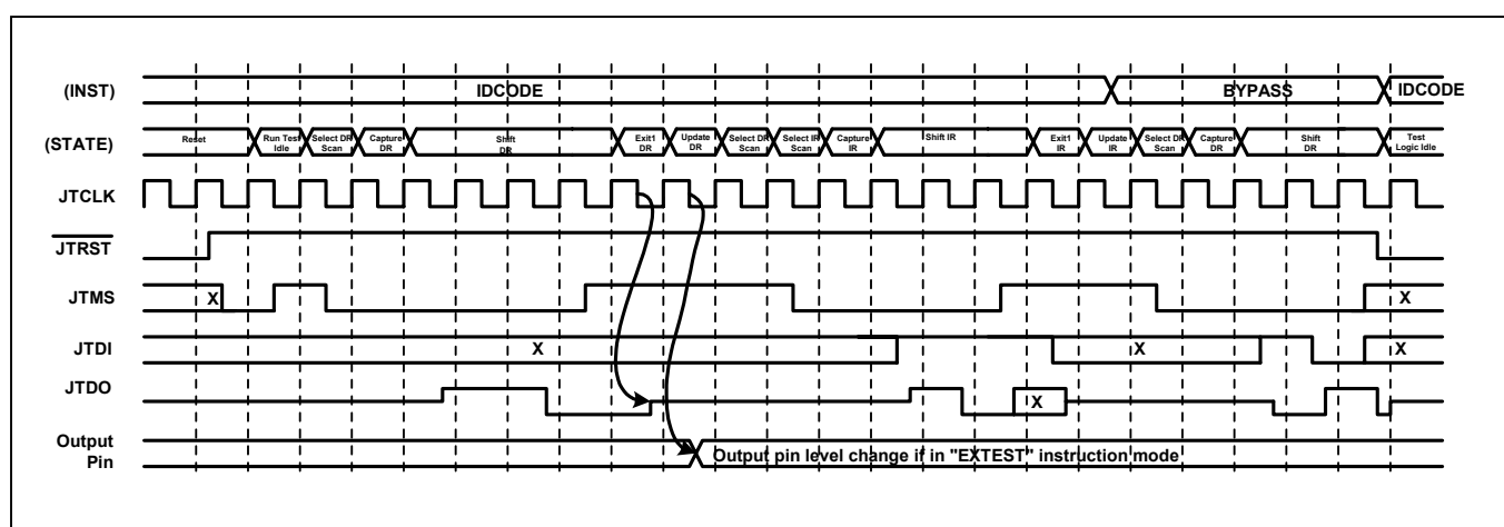
Figure 13-3. JTAG Functional Timing
