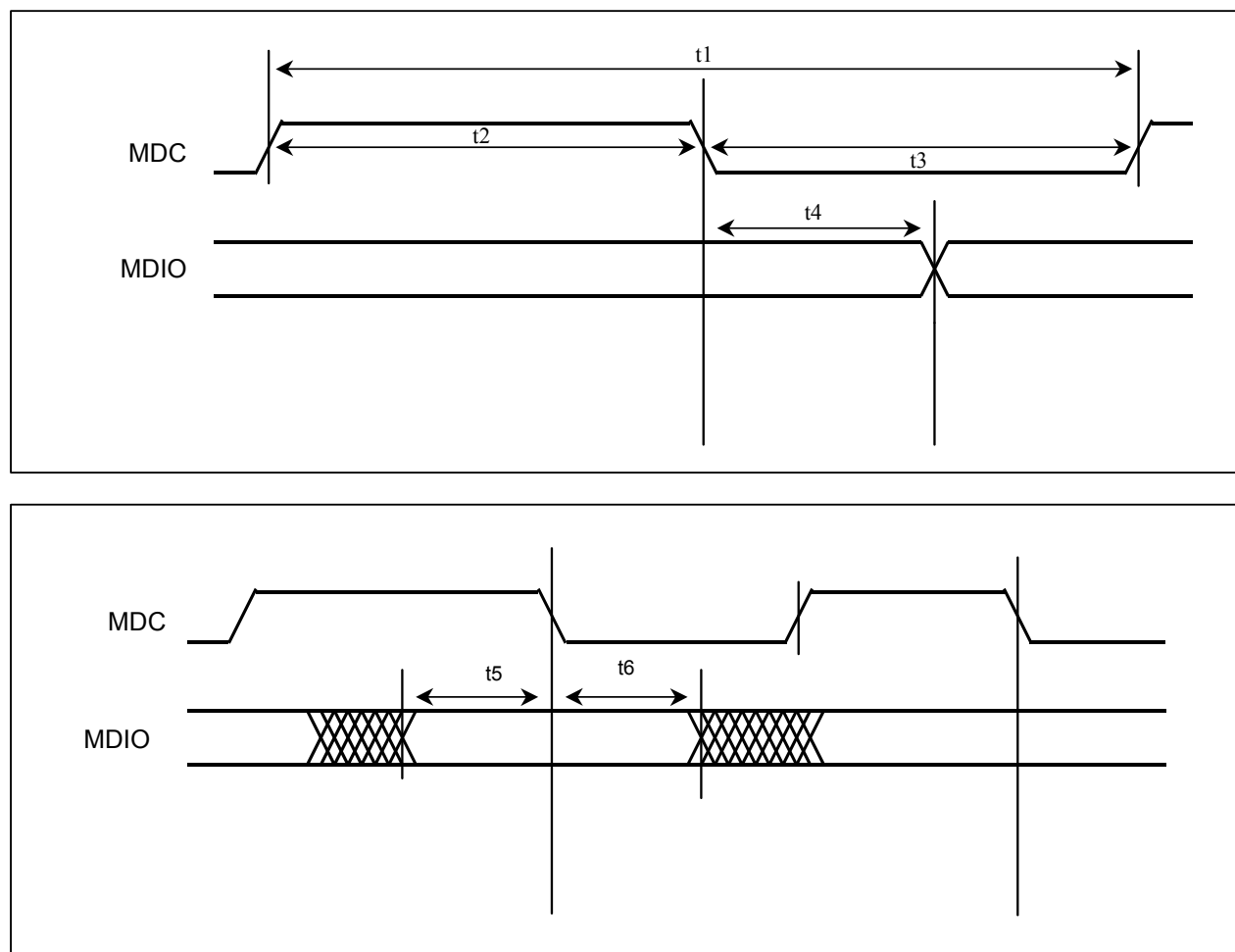
Figure 12-7. MDIO Interface Timing
