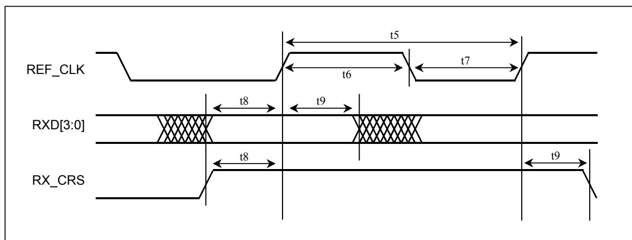
Figure 12-6. Receive RMI Interface Timing
