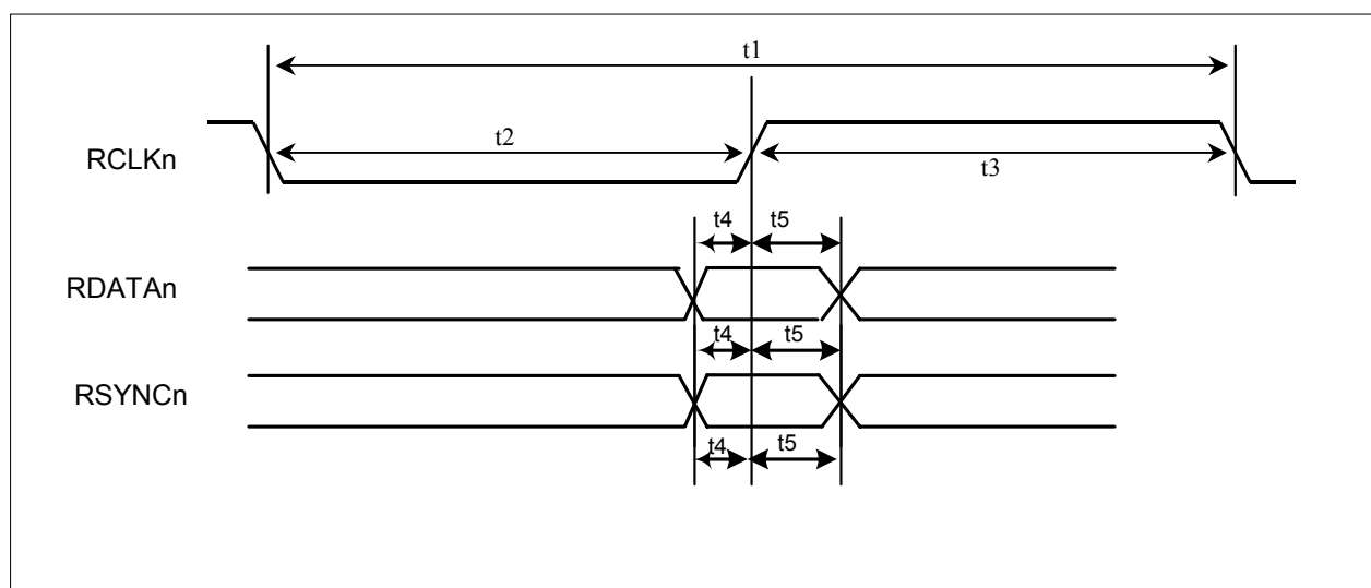
Figure 12-9. Receive WAN Timing (Noninverted RCLK)
