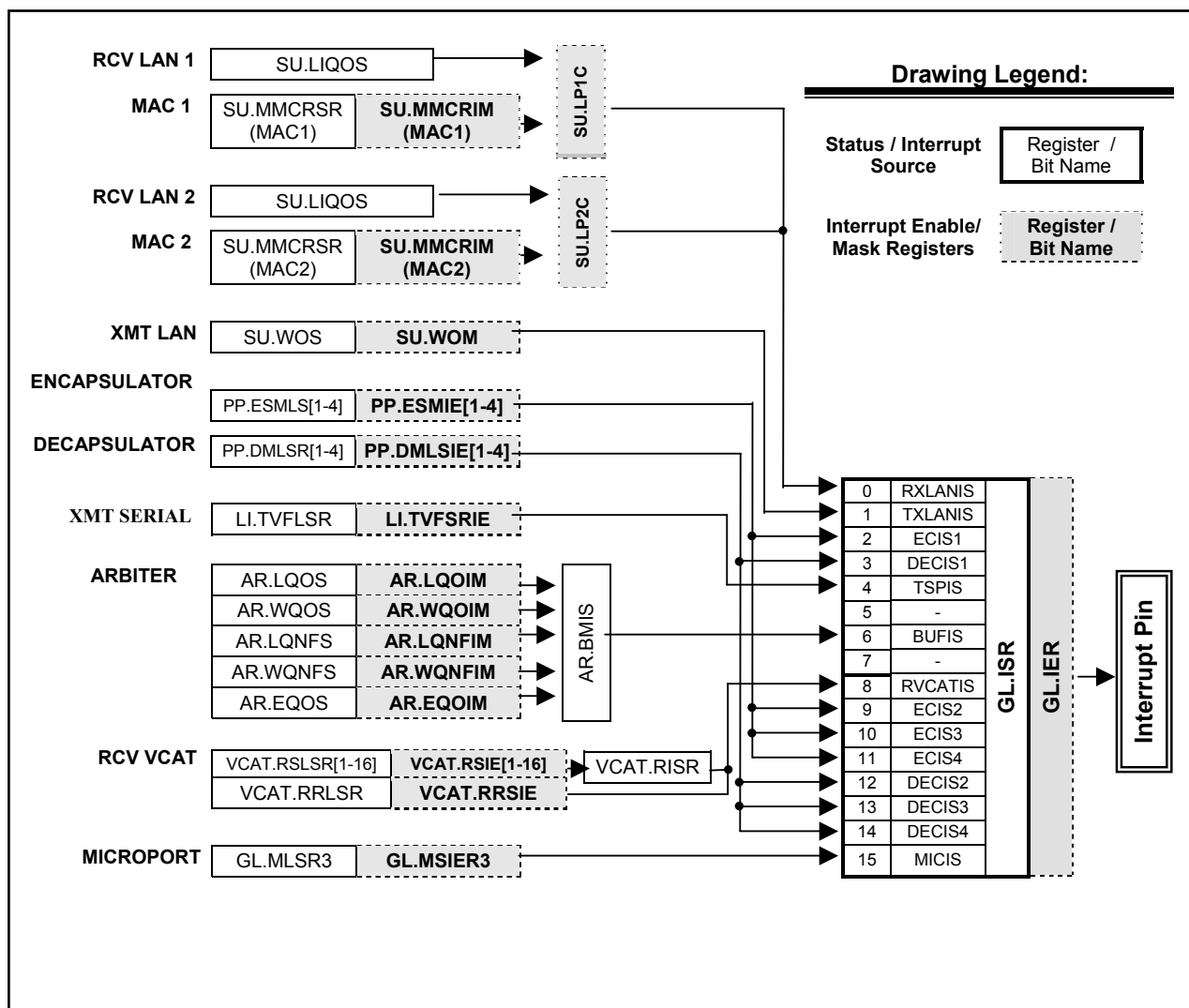
Figure 8-2. Device Interrupt Information Flow Diagram
