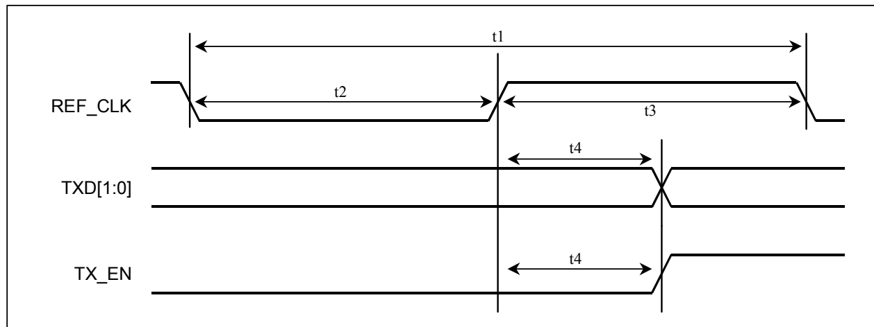
Figure 12-5. Transmit RMII Interface Timing
