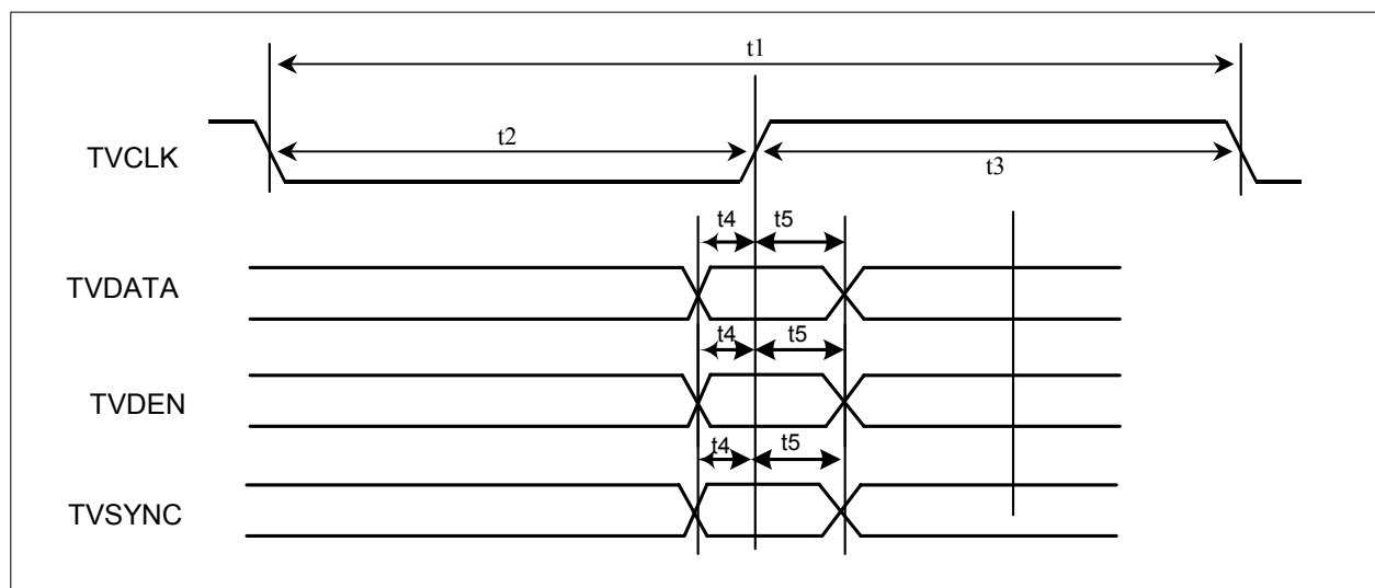
Figure 12-10. Transmit Voice Port Interface Timing
