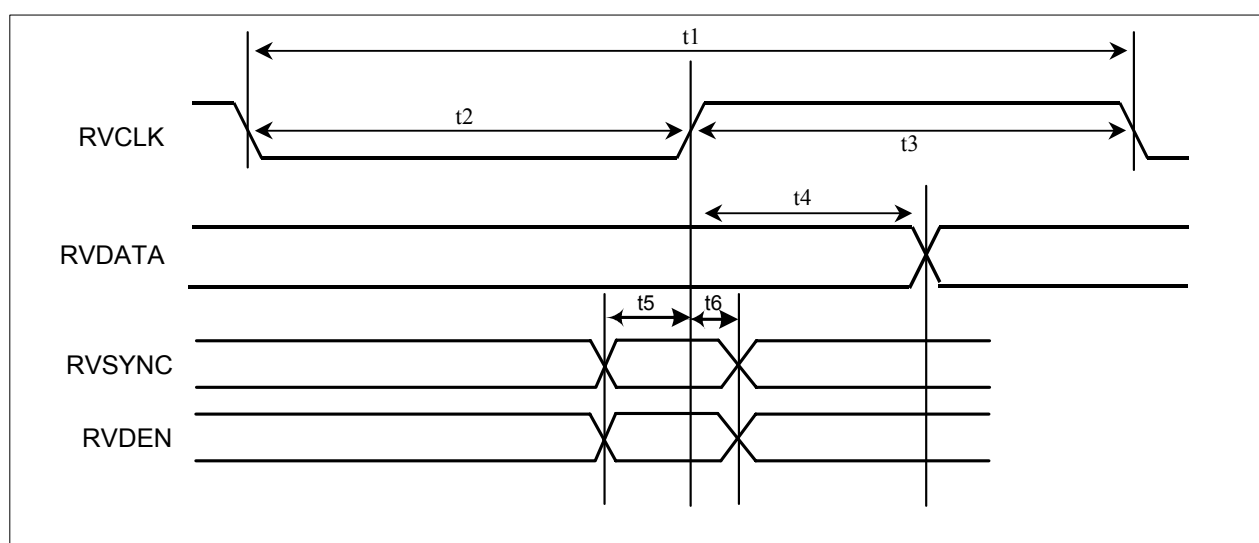
Figure 12-11. Receive Voice Port Interface Timing
