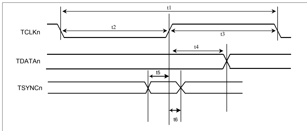
Figure 12-8. Transmit WAN Timing (Noninverted TCLK)
