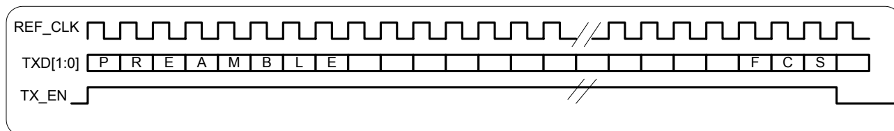
Figure 11-23. RMII Transmit Interface Functional Timing
