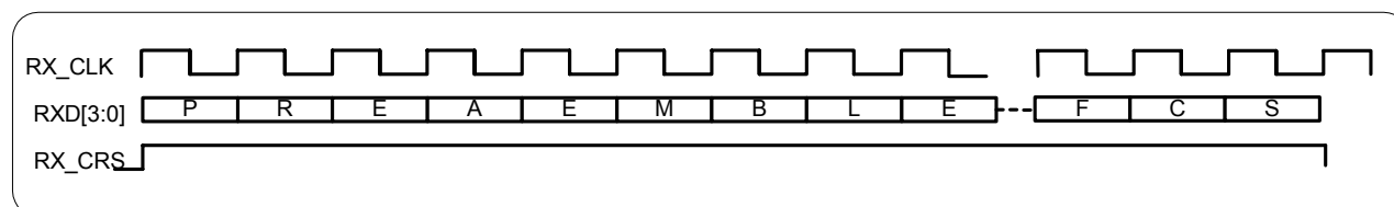
Figure 11-22. MII Receive Functional Timing
