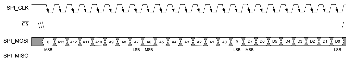
Figure 11-6. SPI Serial Port Access For Write Mode, SPI_CPOL = 1, SPI_CPHA = 0
