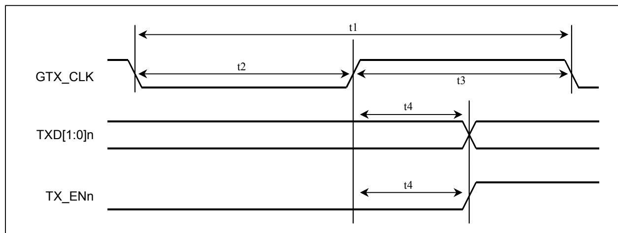
Figure 12-1. Transmit GMII Interface Timing
