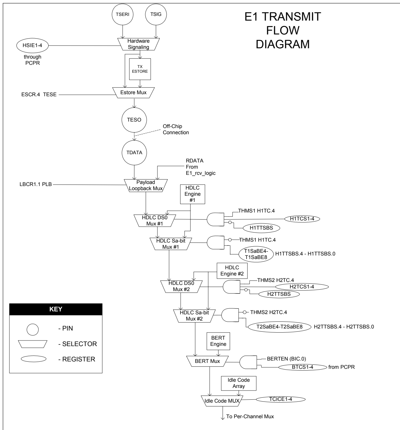
Figure 11-3. E1 Transmit Flow Diagram
