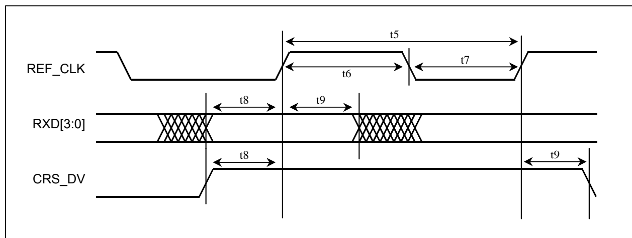
Figure 14-4. Receive RMII Interface Timing
