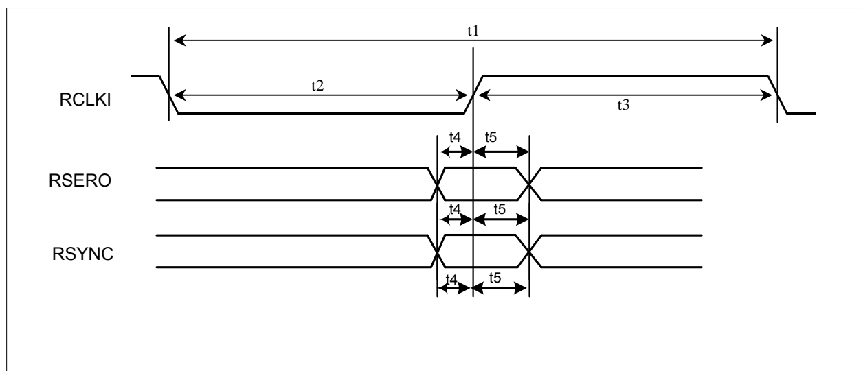
Figure 14-7. Receive WAN Timing
