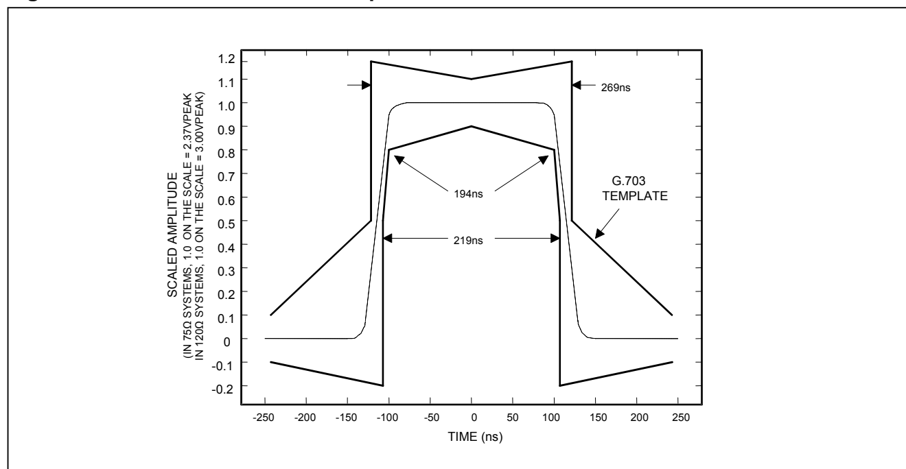
Figure 10-9. E1 Transmit Pulse Template
