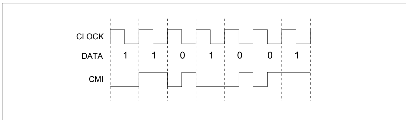
Figure 10-7. CMI Coding
