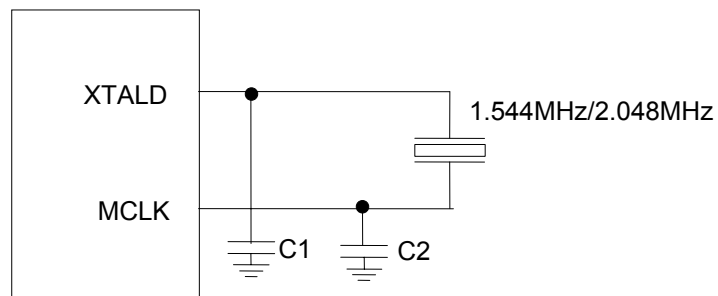
Figure 10-15. Optional Crystal Connections
