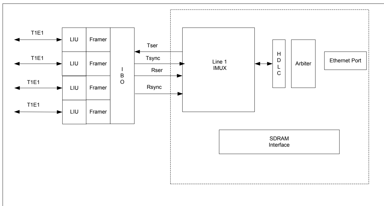
Figure 9-4. Diagram of Data Transmission with IMUX Operation
