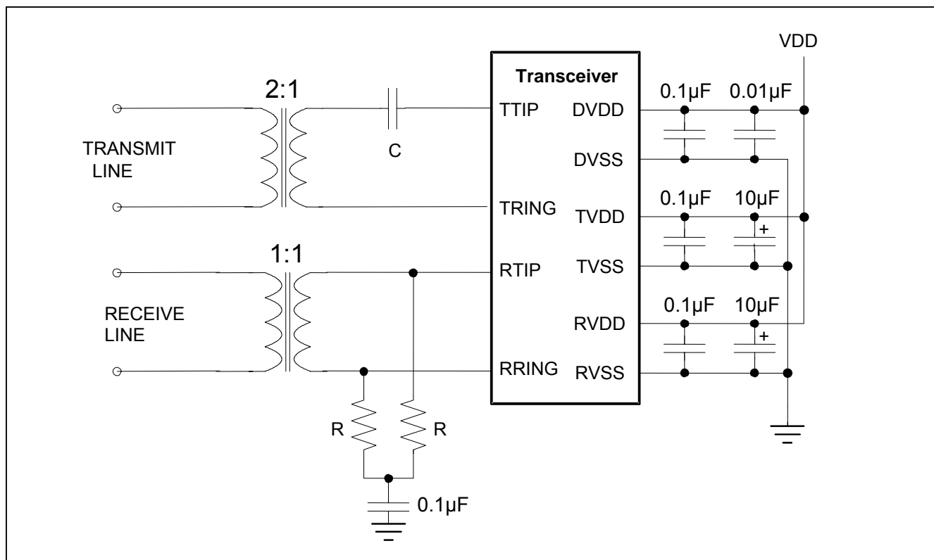
Figure 10-8. Basic Interface
