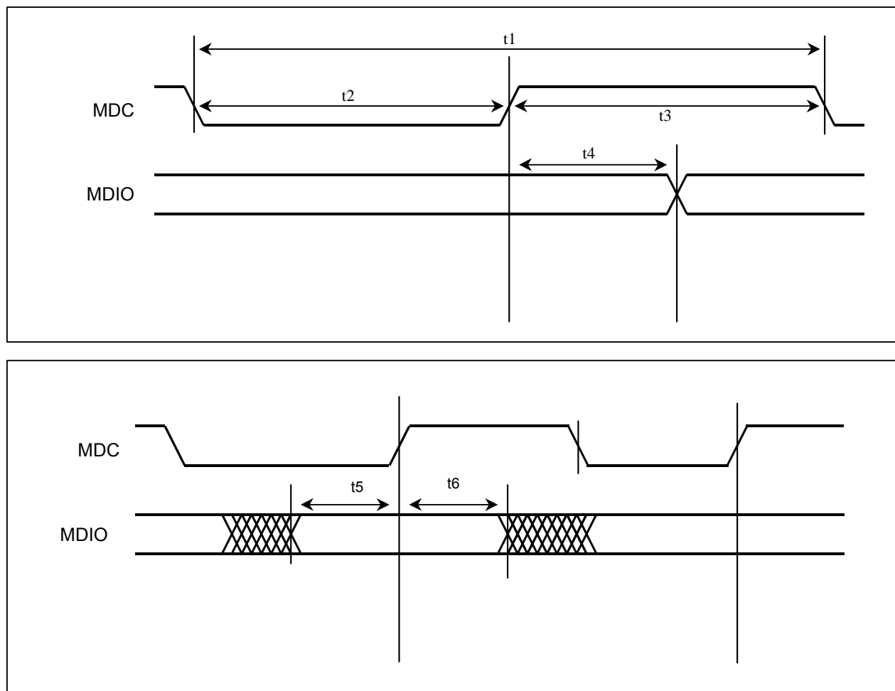
Figure 14-5. MDIO Interface Timing
