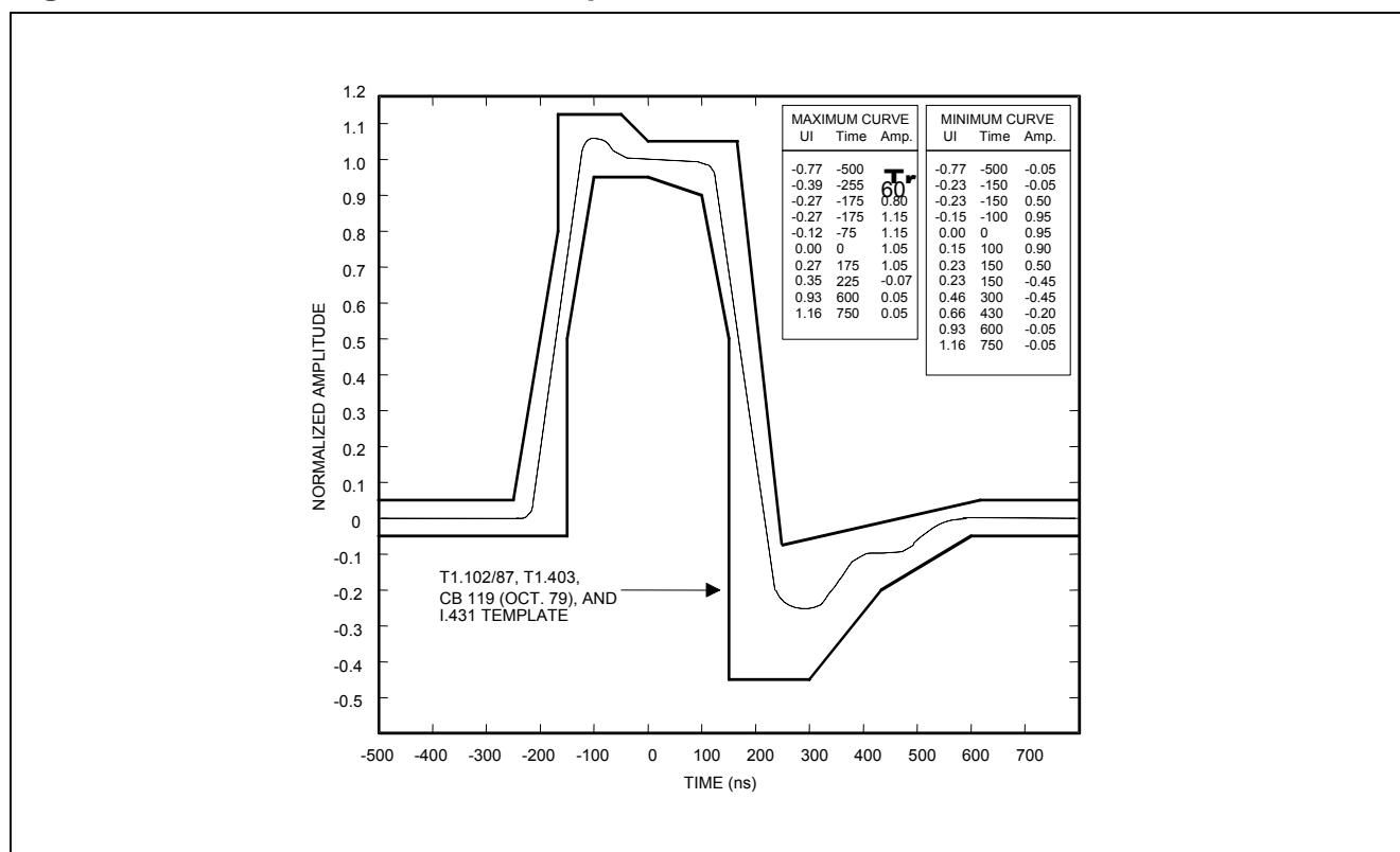
Figure 10-10. T1 Transmit Pulse Template
