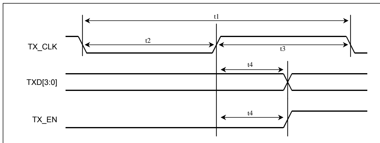
Figure 14-1. Transmit MII Interface Timing
