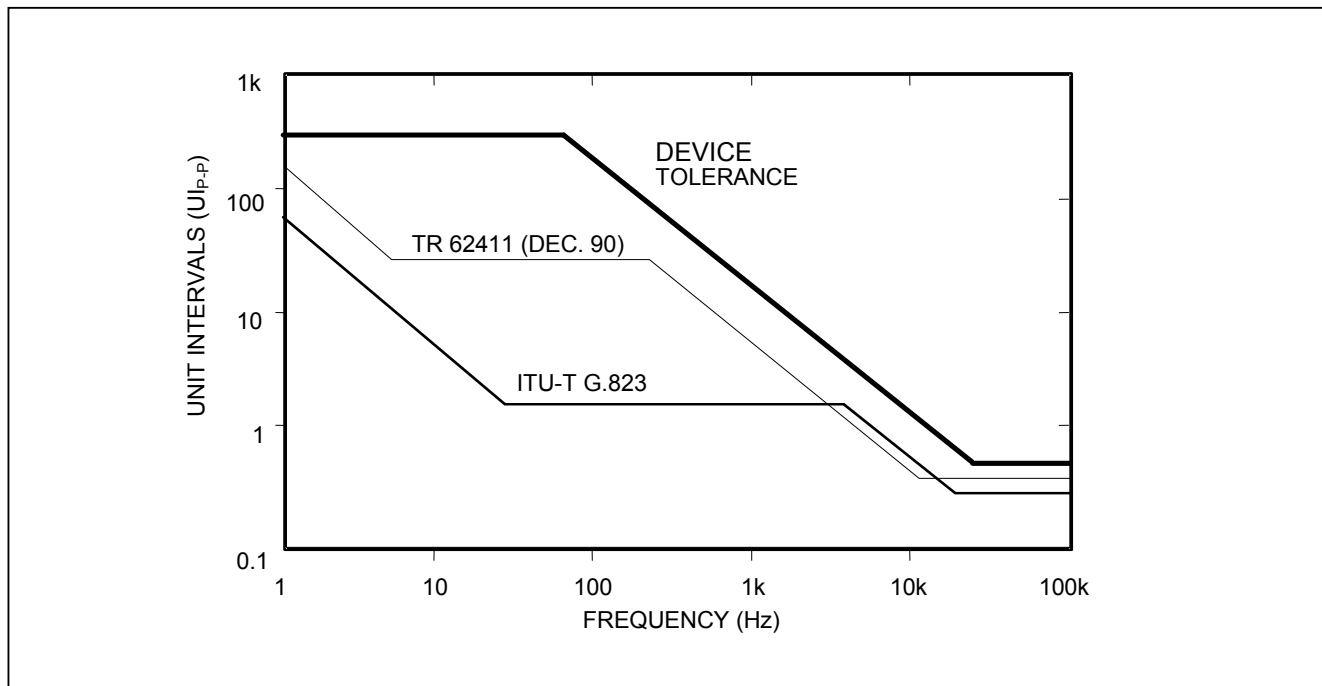
Figure 10-11. Jitter Tolerance
