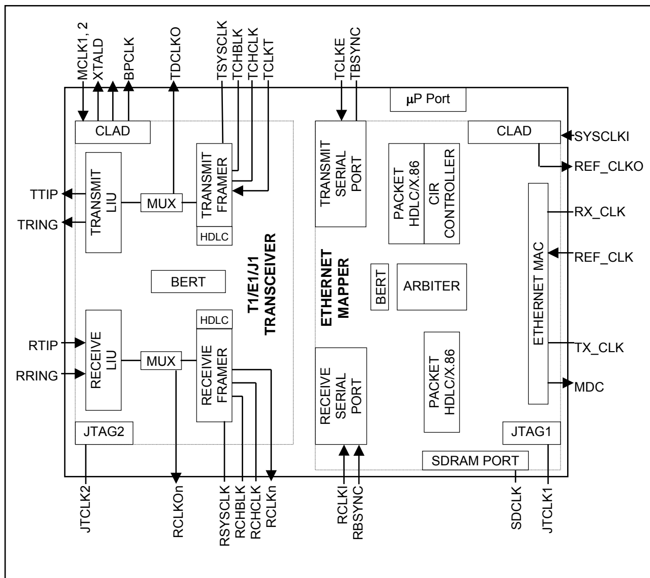
Figure 9-1. Clocking for the DS33R41
