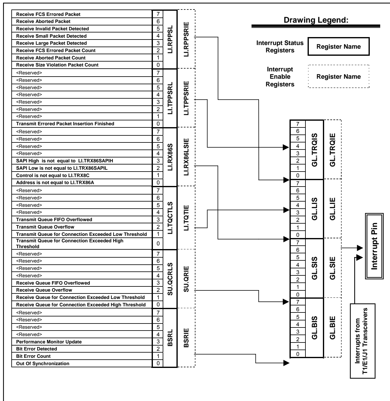
Figure 9-2. Device Interrupt Information Flow Diagram
