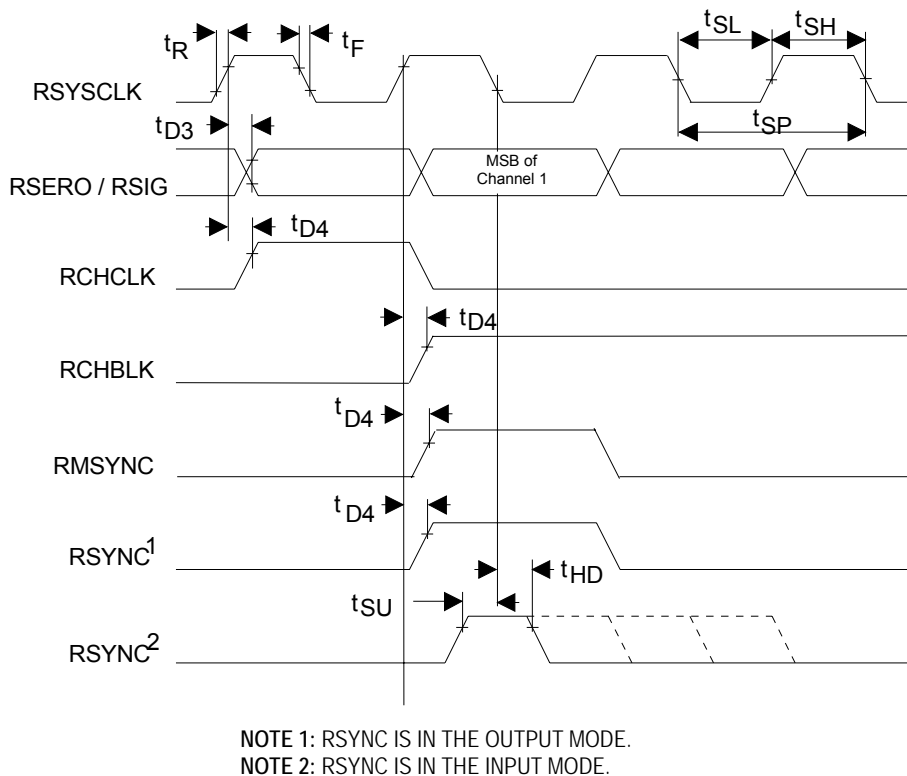
Figure 14-18. Receive Line Interface Timing
