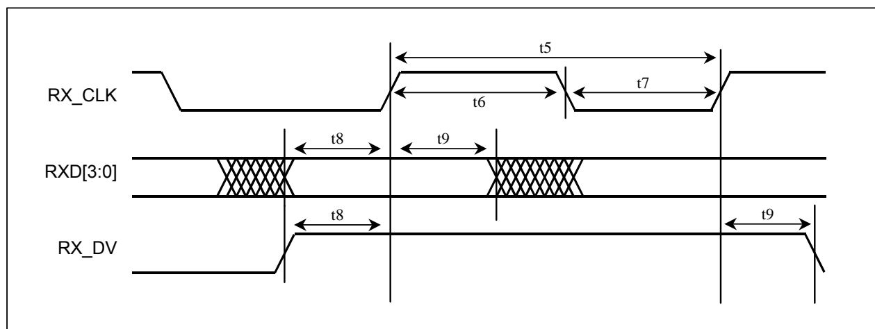
Figure 14-2. Receive MII Interface Timing
