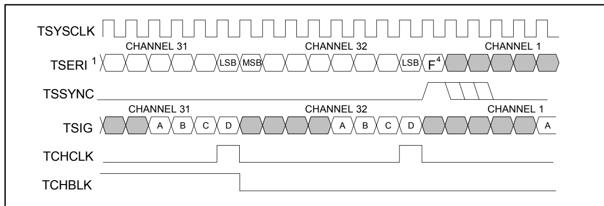
Figure 13-22. Transmit Side Boundary Timing, TSYSClk = 2.048MHz (With Elastic Store Enabled)
