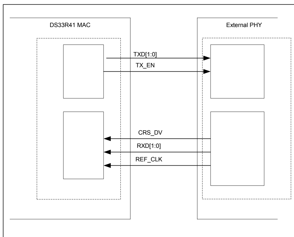
Figure 9-10. RMII Interface
