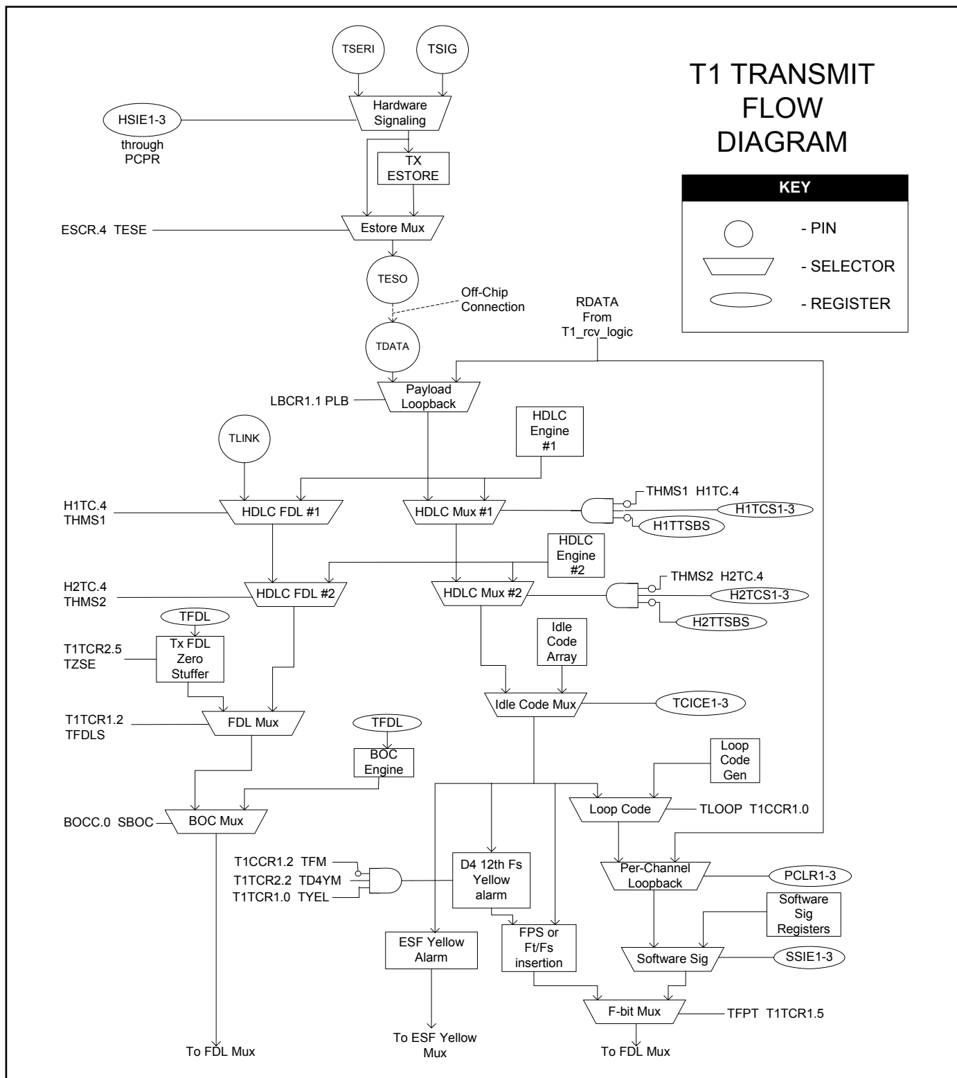
Figure 11-2. T1/J1 Transmit Flow Diagram
