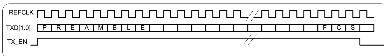
Figure 13-4. RMII Transmit Interface Functional Timing
