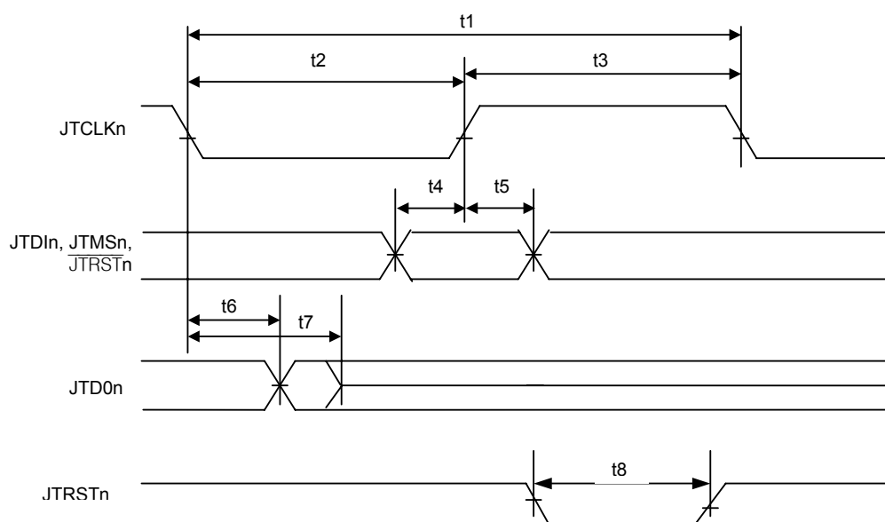
Figure 14-13. JTAG Interface Timing
