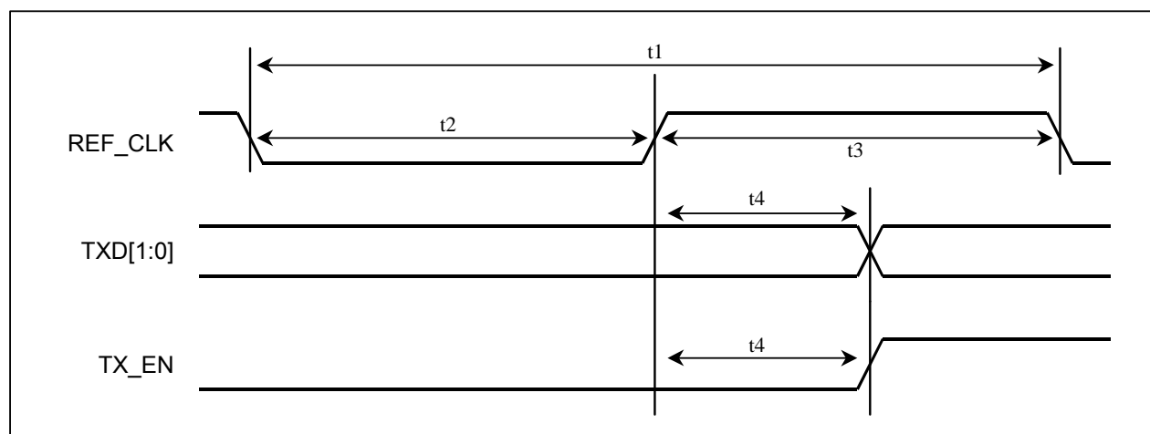
Figure 14-3. Transmit RMII Interface Timing
