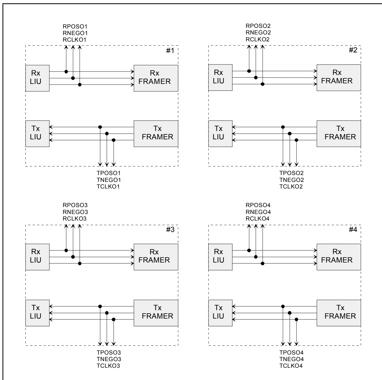
Figure 6-3. Framer/LIU Interim Signals
