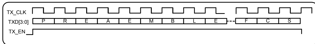
Figure 13-1. MII Transmit Functional Timing
