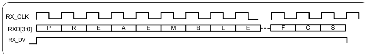
Figure 13-3. MII Receive Functional Timing
