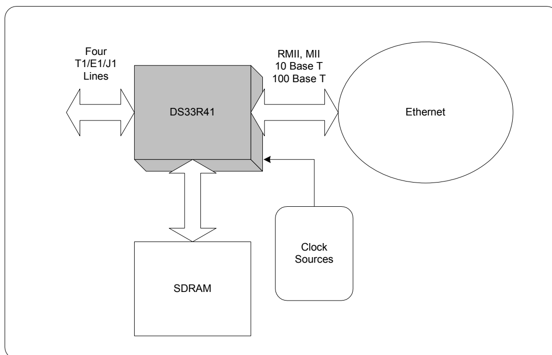
Figure 3-1. Quad T1E1 SCT to DS33R41
