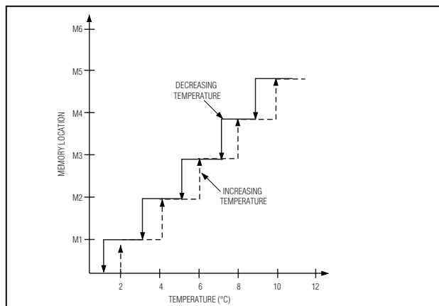
Figure 4. Look-Up Table Temperature Hysteresis
