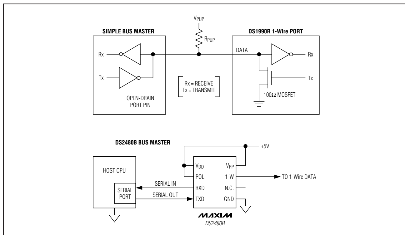
Figure 4. Hardware Configuration
