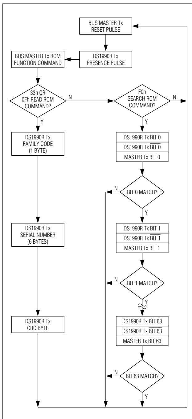
Figure 5. ROM Functions Flowchart
