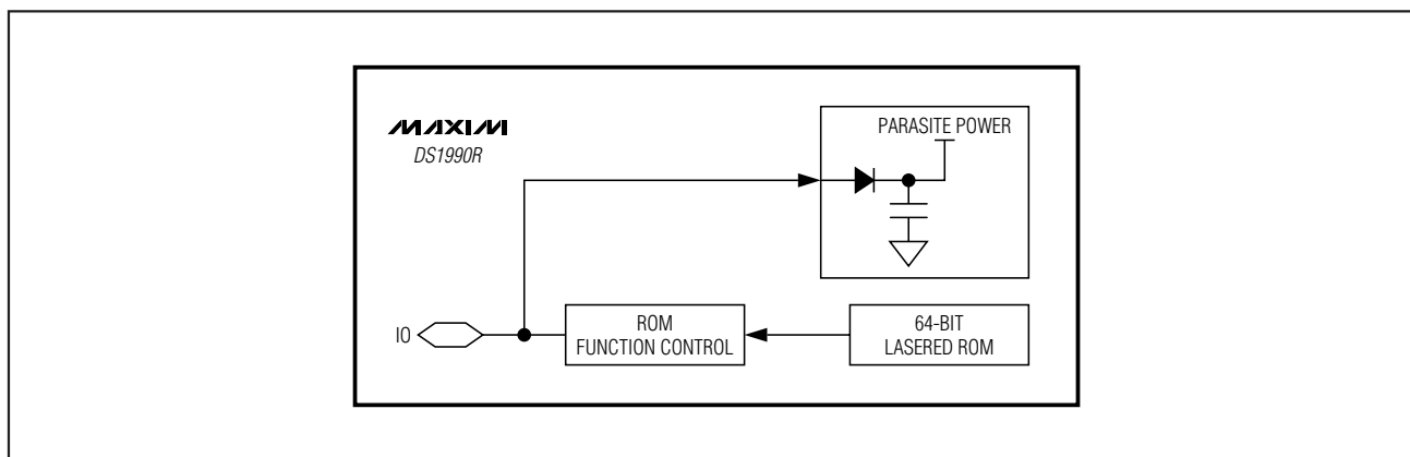
Figure 1. Block Diagram
