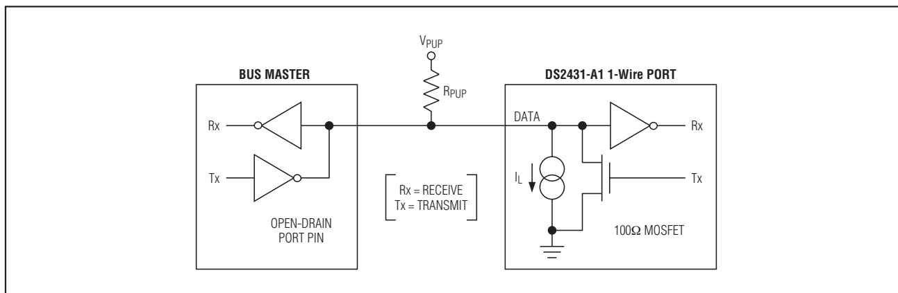
Figure 8. Hardware Configuration
