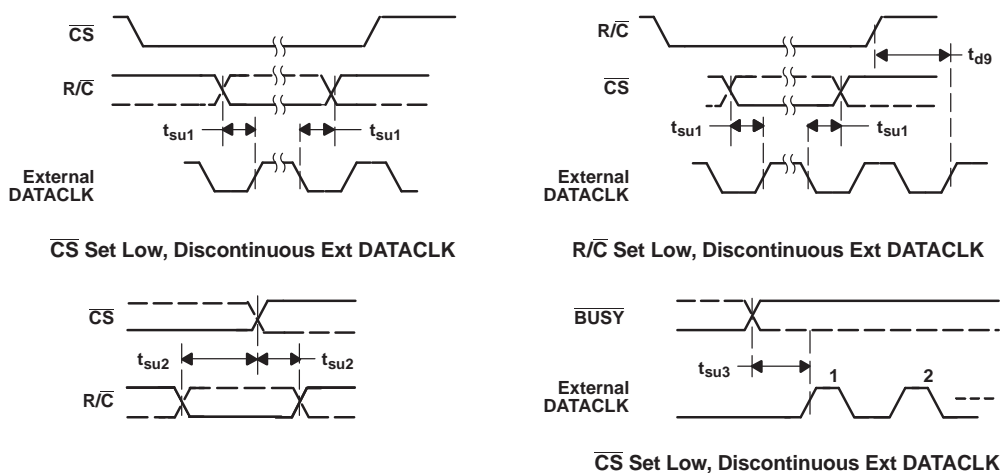
Figure 35. Critical Timing
