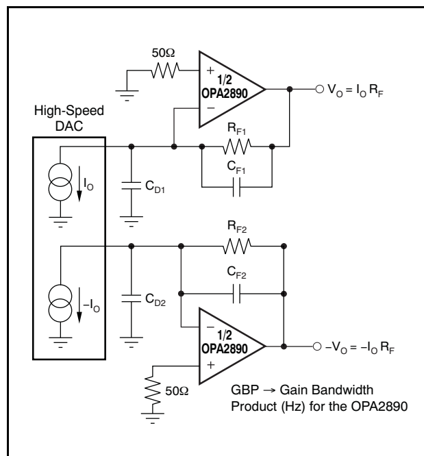
Figure 53. DAC Transimpedance Amplifier
