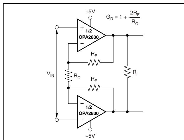
Figure 52. Differential Noninverting Specification and Test Circuit
