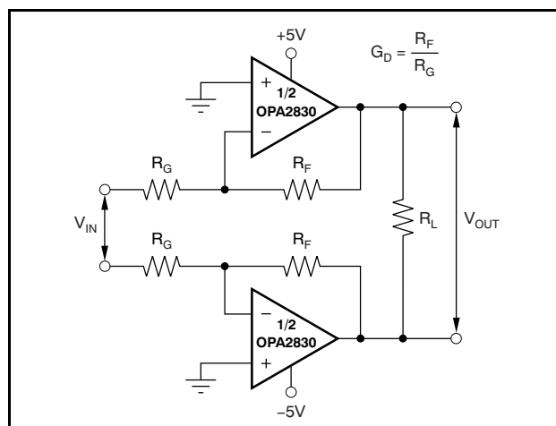
Figure 51. Differential Inverting Specification and Test Circuit
