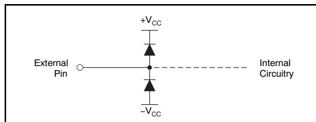
Figure 63. Internal ESD Protection
