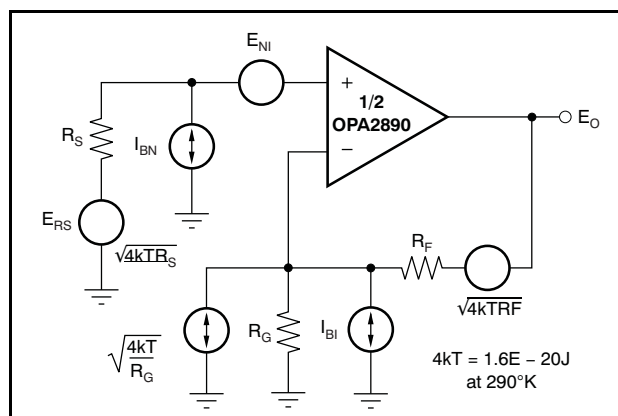
Figure 60. Op Amp Noise Analysis Model
