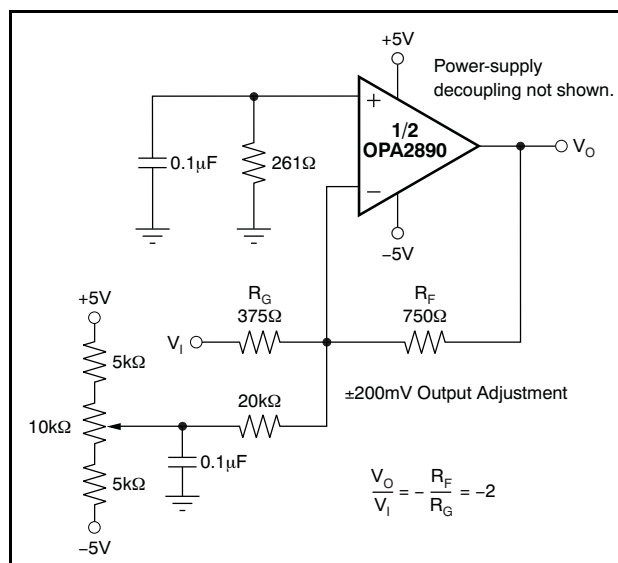
Figure 61. DC-Coupled, Inverting Gain of -2, with Offset Adjustment
