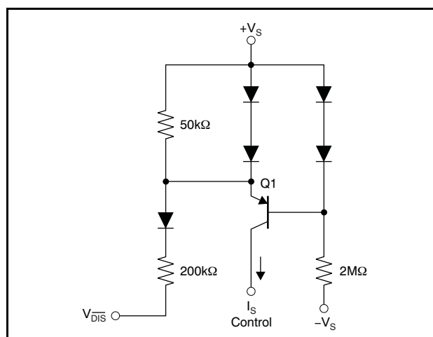
Figure 62. Simplified Disable Control Circuit
