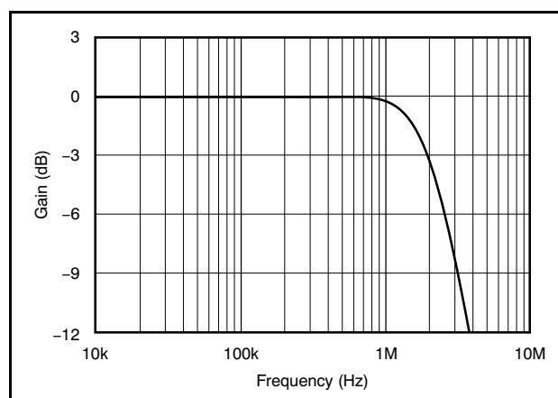
Figure 57. Multiple Feedback Filter Frequency Response
