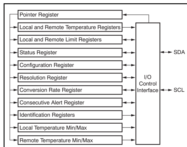
Figure 12. Internal Register Structure
