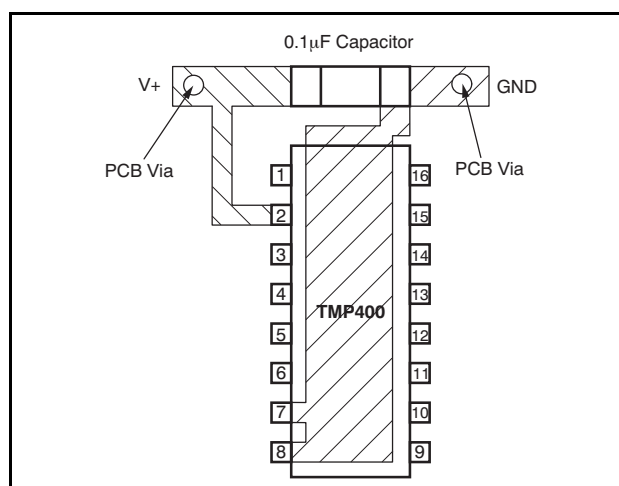
Figure 20. Suggested Bypass Capacitor Placement
