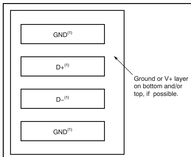
Figure 19. Example Signal Traces
