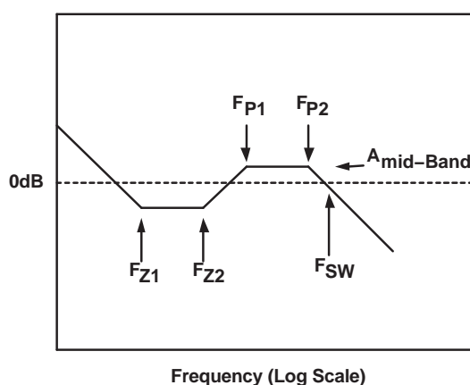
Figure 21. Error Amplifier Frequency Response Straight Line Approximation
