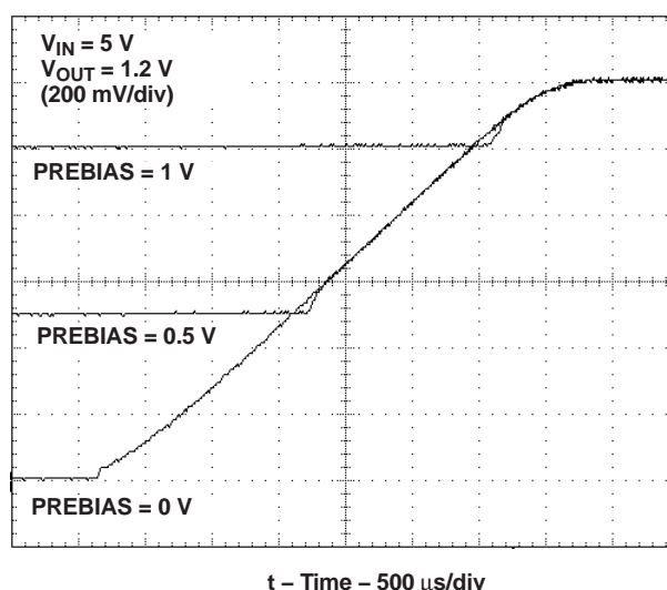
Figure 17. Startup Waveforms; VREFIN = 0.6 V
