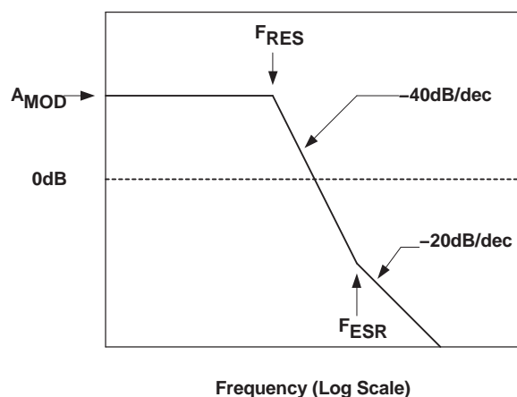
Figure 20. Power Stage Frequency Response Straight Line Approximation
