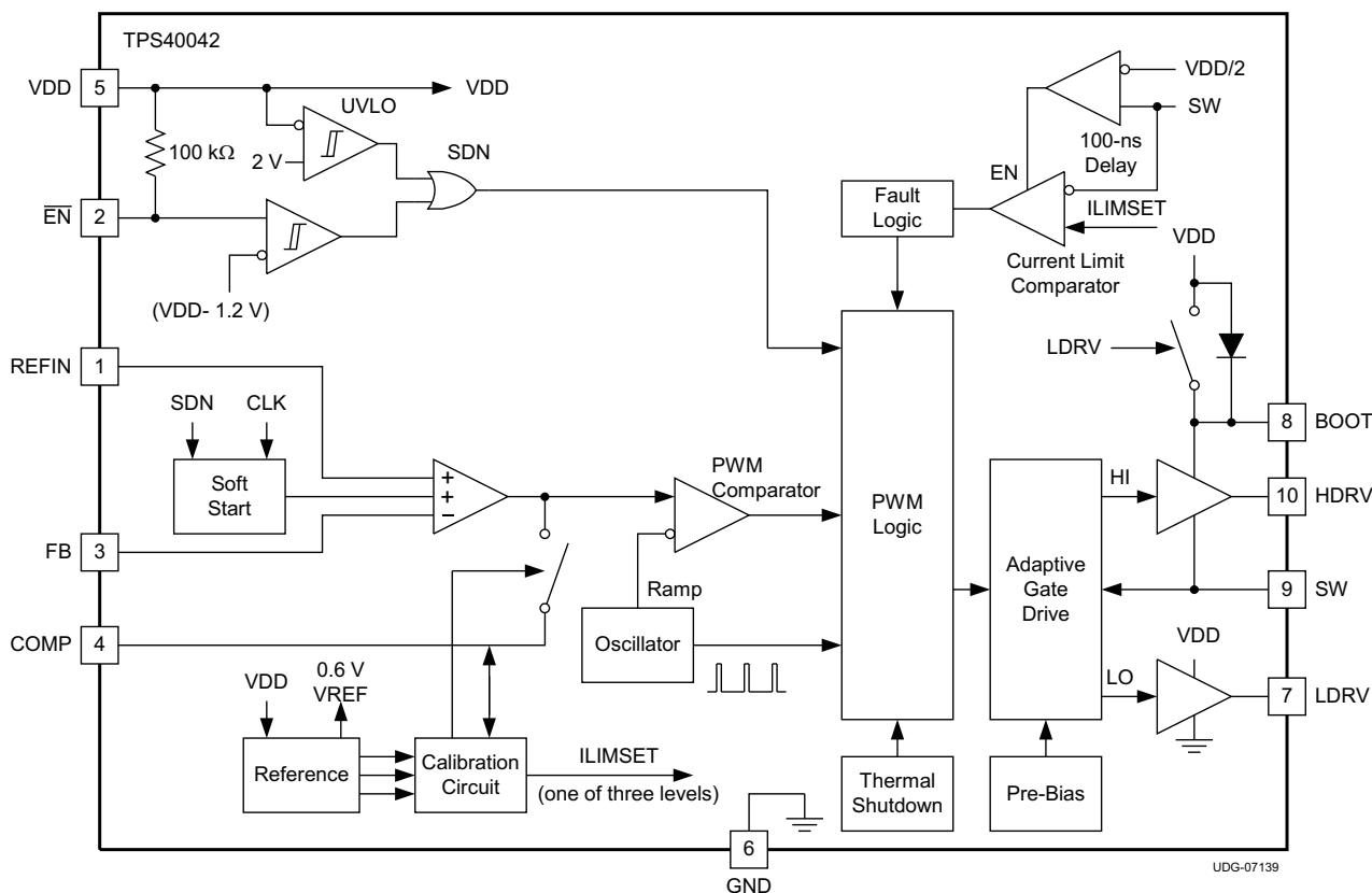
Figure 14. Functional Block Diagram
