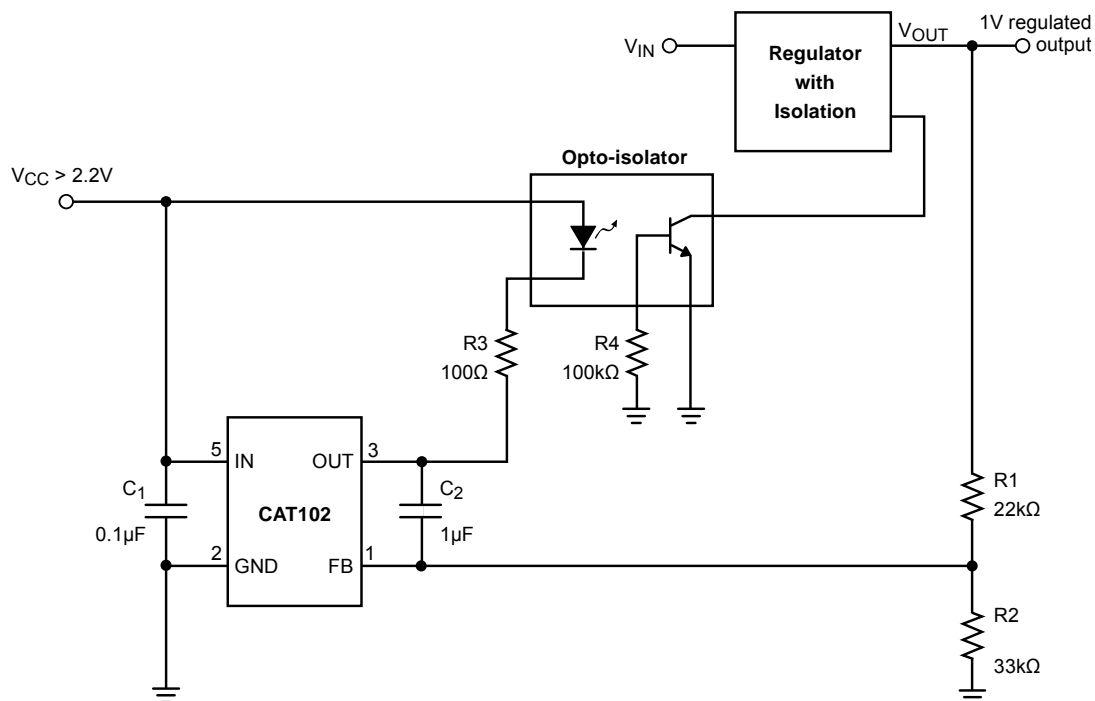
Figure 2. Opto-Feedback Application Circuit
