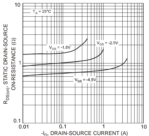
Fig. 6 Static Drain-Source On-Resistance vs. Drain-Source Current
