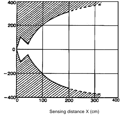
Through-Beam Type E3SA-2C43A With Slit
