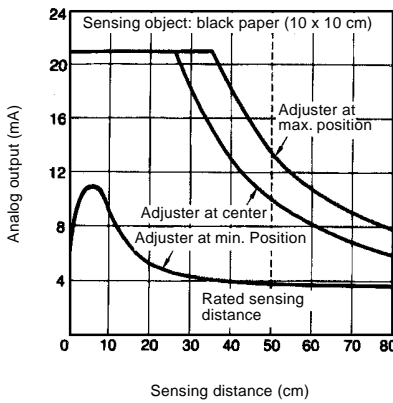
Diffuse Reflective Type E3SA-DS50C43A (white object)
