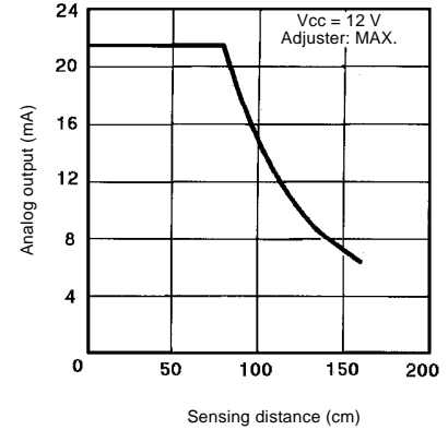
Polarized Retroreflective Type E3SA-RS50C43A
