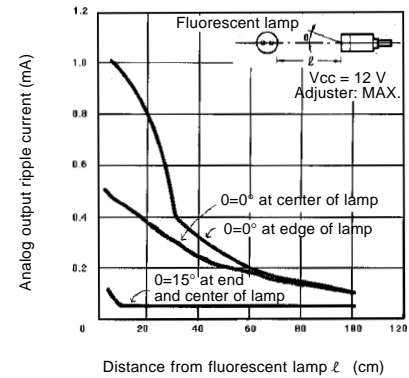
Retroreflective Type E3SA-RS50C43A
