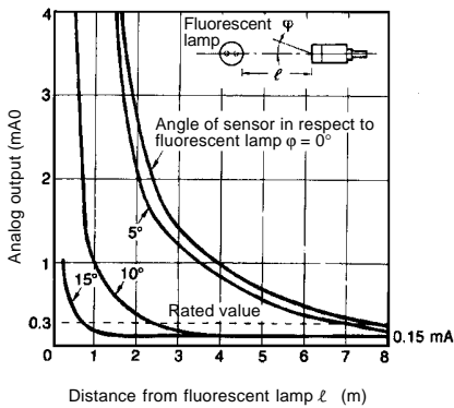
Diffuse Reflective Type E3SA-DS50C43A
