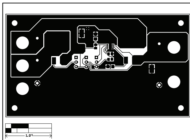
Figure 3. MAX6496 EV Kit PCB Layout—Component Side
