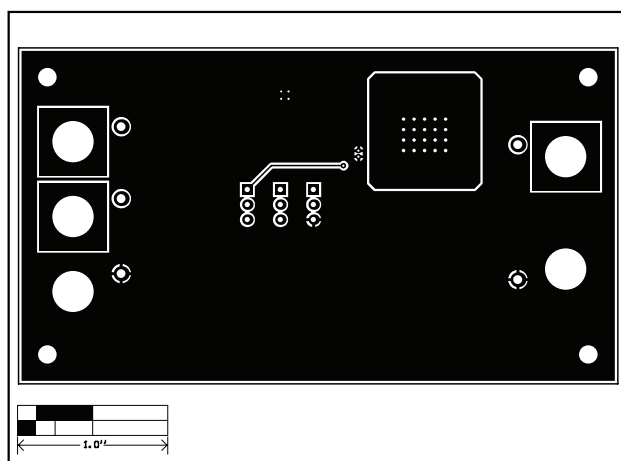
Figure 4. MAX6496 EV Kit PCB Layout—Solder Side
