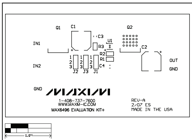
Figure 2. MAX6496 EV Kit Component Placement Guide—Component Side
