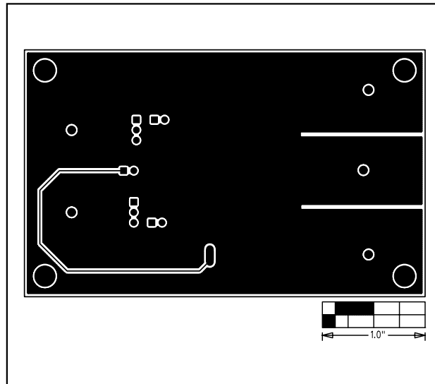
Figure 4. MAX7443 EV Kit PCB Layout—Solder Side
