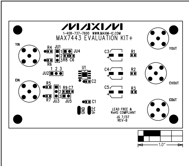
Figure 2. MAX7443 EV Kit Component Placement Guide—Top Silkscreen
