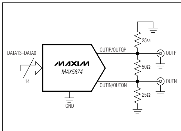
Figure 7. Differential Output Configuration
