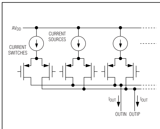
Figure 3. Simplified Analog Output Structure
