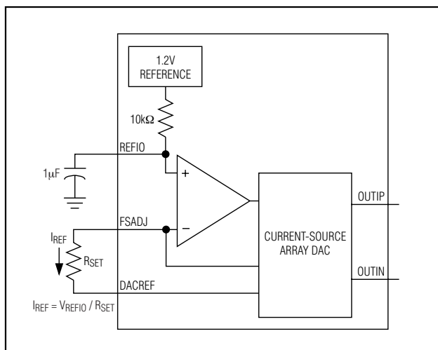
Figure 2. Reference Architecture, Internal Reference Configuration
