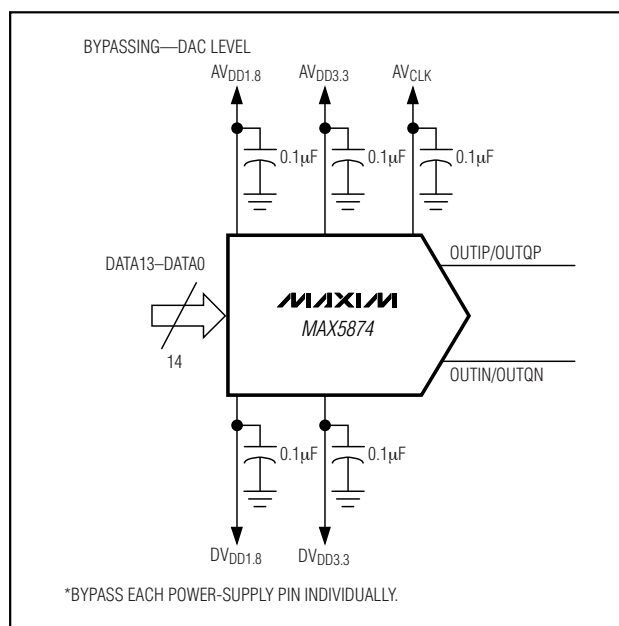
Figure 8. Recommended Power-Supply Decoupling and Bypassing Circuitry
