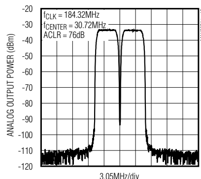
ACLR FOR WCDMA MODULATION, TWO CARRIERS
