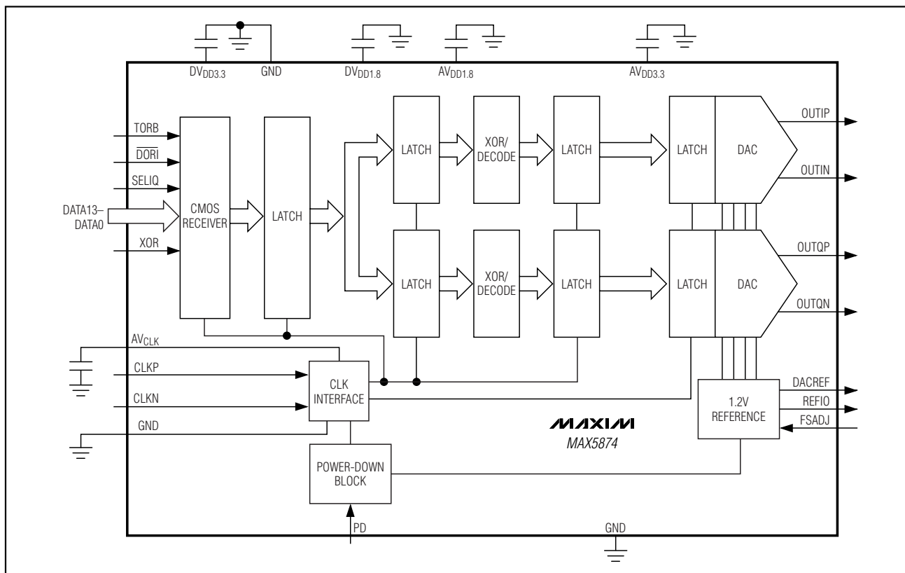
Figure 1. MAX5874 High-Performance, 14-Bit, Dual Current-Steering DAC
