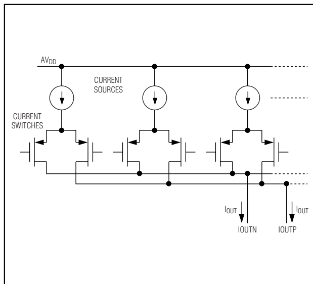
Figure 3. Simplified Analog Output Structure
