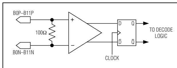
Figure 6. Simplified LVDS-Compatible Input Structure
