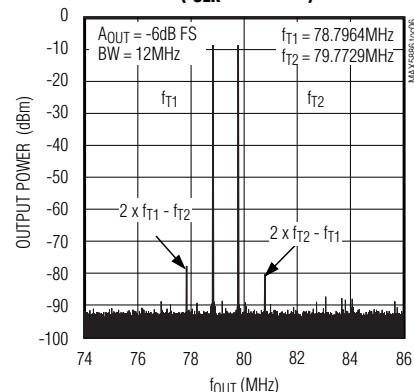
2-TONE INTERMODULATION DISTORTION ( f_{CLK} = 500MHz )
