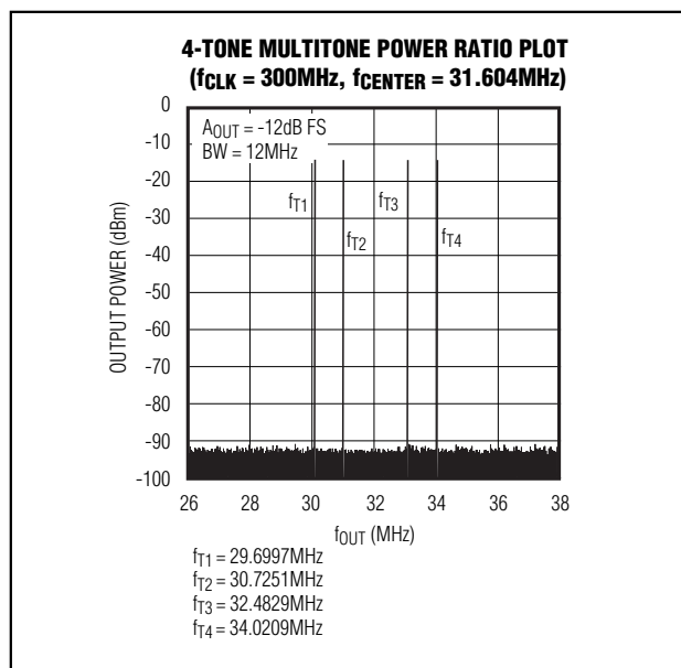
Figure 12. 4-Tone MTPR Test Results
