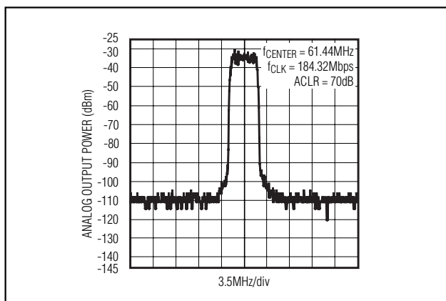
Figure 9. ACLR for W-CDMA Modulation, Single Carrier
