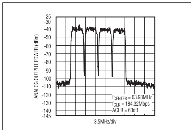
Figure 10. ACLR for W-CDMA Modulation, Four Carriers
