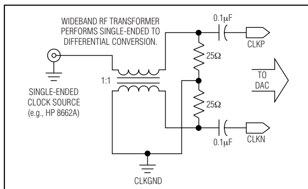
Figure 4. Differential Clock Signal Generation
