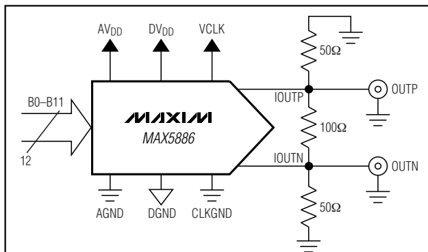
Figure 8. MAX5886 Differential Output Configuration
