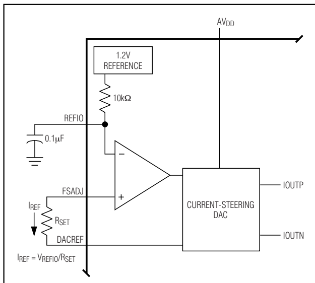
Figure 2. Reference Architecture, Internal Reference Configuration
