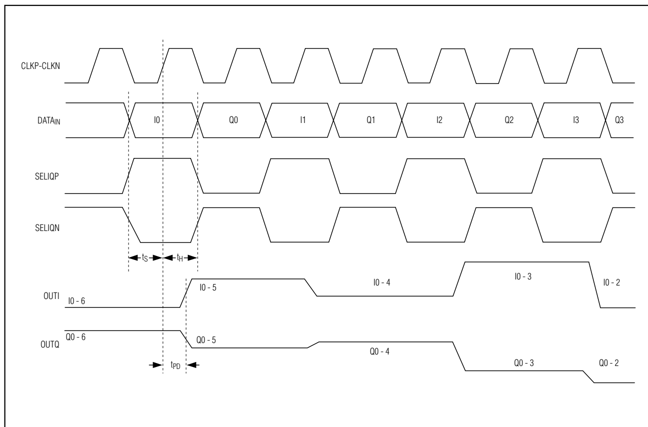
Figure 4. Timing Diagram
