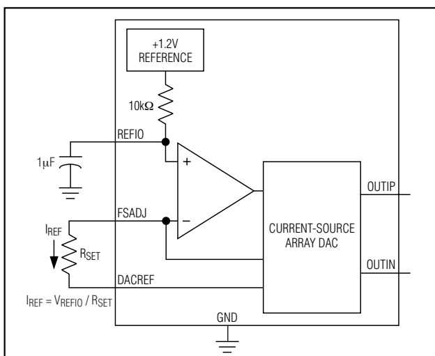
Figure 2. Reference Architecture, Internal Reference Configuration
