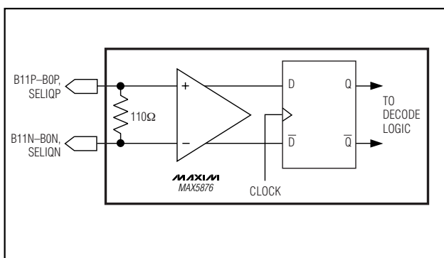
Figure 5. Simplified LVDS-Compatible Digital Input Structure
