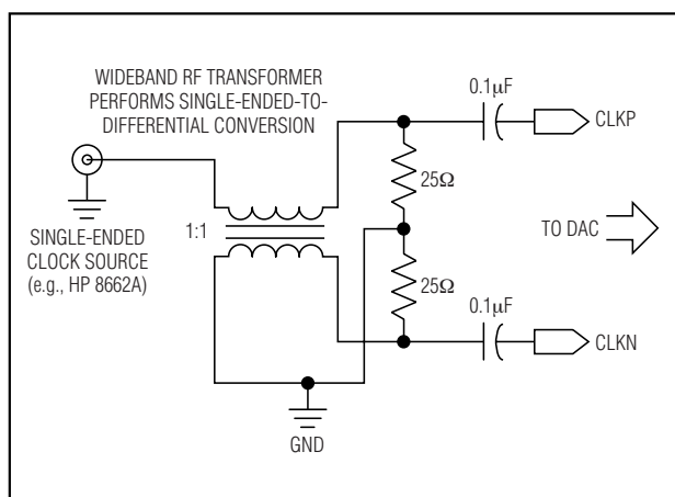
Figure 6. Differential Clock-Signal Generation
