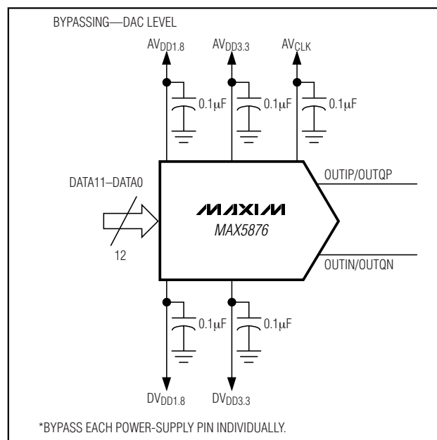
Figure 9. Recommended Power-Supply Decoupling and Bypassing Circuitry
