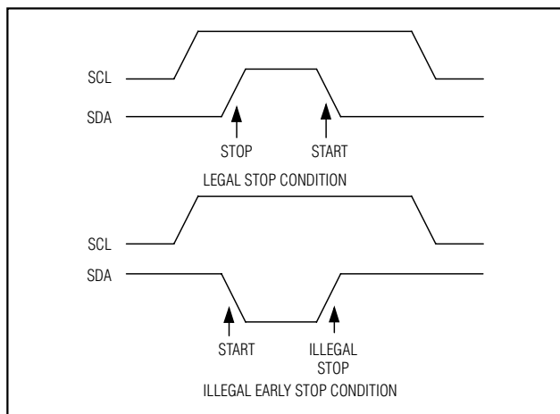
Figure 6. Early STOP Conditions
