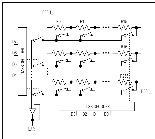
Figure 3. DAC Simplified Circuit Diagram
