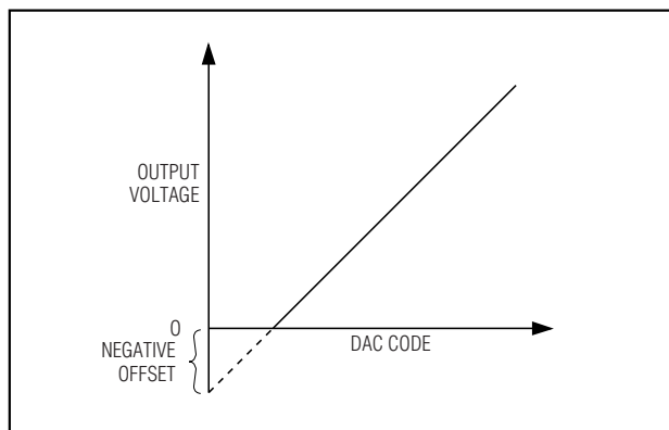
Figure 10. Effect of Negative Offset (Single Supply)
