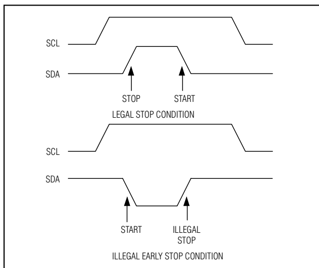
Figure 3. Early STOP Conditions
