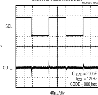
DIGITAL FEEDTHROUGH
