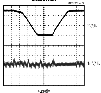
CROSSTALK
