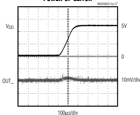
POWER-UP GLITCH
