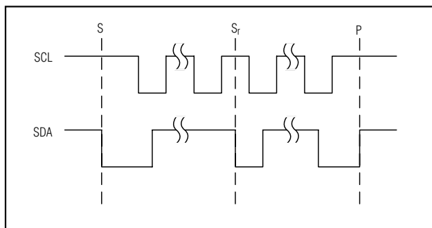
Figure 2. START and STOP Conditions
