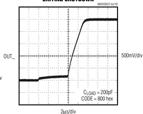
EXITING SHUTDOWN
