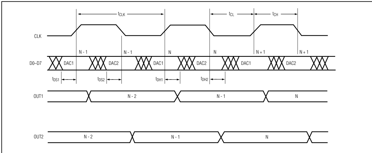
Figure 4. Timing Diagram
