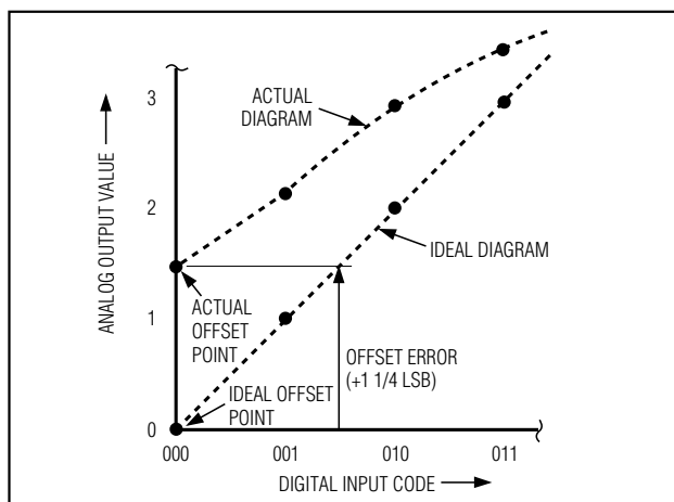
Figure 5c. Offset Error
