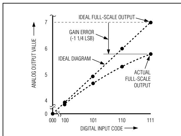
Figure 5d. Gain Error
