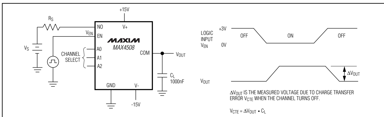
Figure 5. Charge Injection
