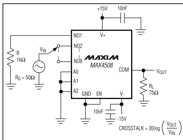
Figure 7. Crosstalk
