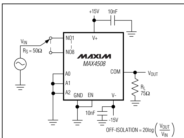
Figure 6. Off-Isolation
