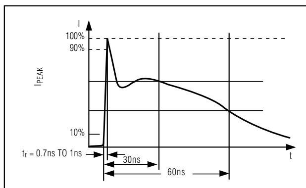
Figure 14. IED 1000-4-2 ESD Generator Current Waveform
