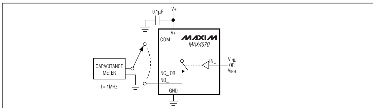
Figure 6. Channel Off-/On-Capacitance
