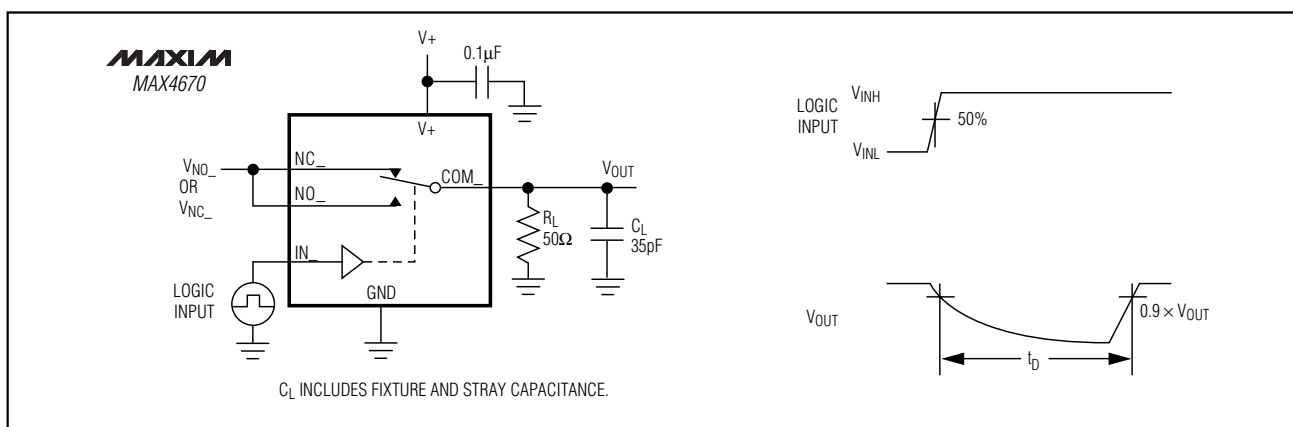
Figure 3. Break-Before-Make Intervals
