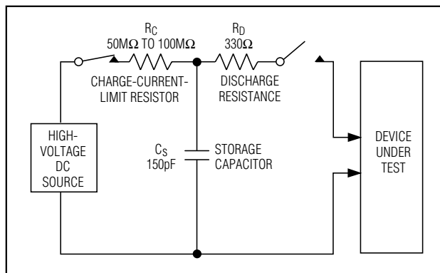
Figure 13. IEC 1000-4-2 ESD Test Model
