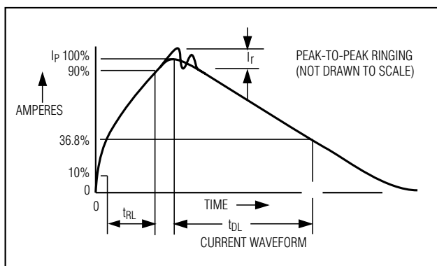
Figure 12. Human Body Model Current Waveform
