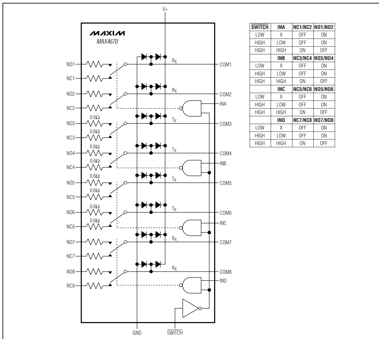
Figure 1. Functional Diagram
