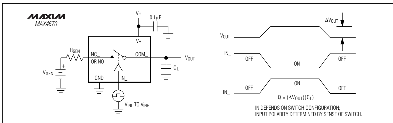
Figure 4. Charge Injection
