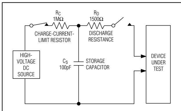
Figure 11. Human Body ESD Test Model
