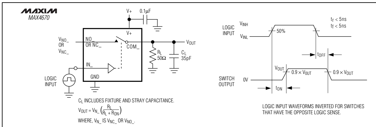
Figure 2. Switching Time
