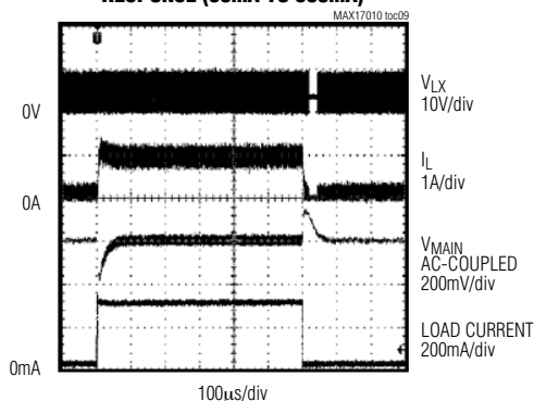
STEP-UP CONVERTER LOAD-TRANSIENT RESPONSE (30mA TO 300mA)
