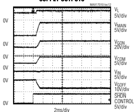
POWER-UP SEQUENCE OF ALL SUPPLY OUTPUTS
