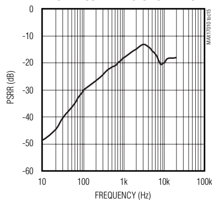
OPERATIONAL AMPLIFIER POWER-SUPPLY REJECTION RATIO
