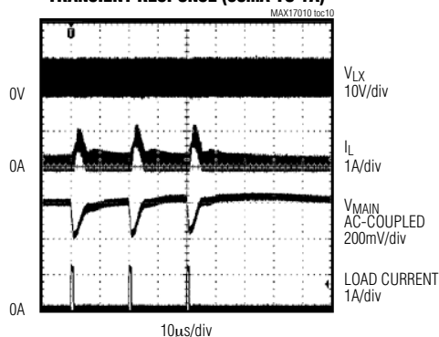
STEP-UP CONVERTER PULSED LOAD-TRANSIENT RESPONSE (30mA TO 1A)
