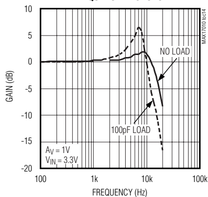
OPERATIONAL AMPLIFIER FREQUENCY RESPONSE
