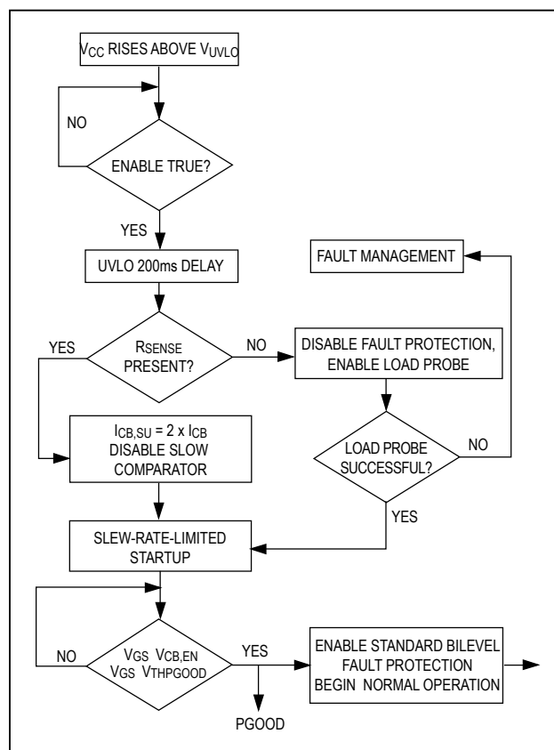
Figure 4. Startup Flow Chart
