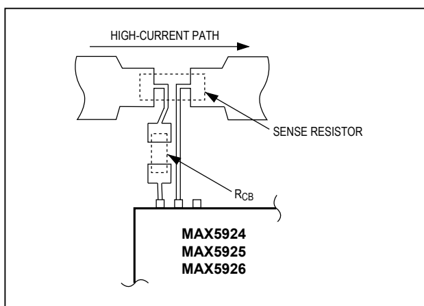
Figure 15. Kelvin Connection for the Current-Sense Resistor
