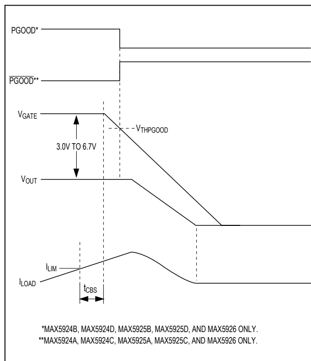
Figure 7. Slow Comparator Response to an Overcurrent Fault
