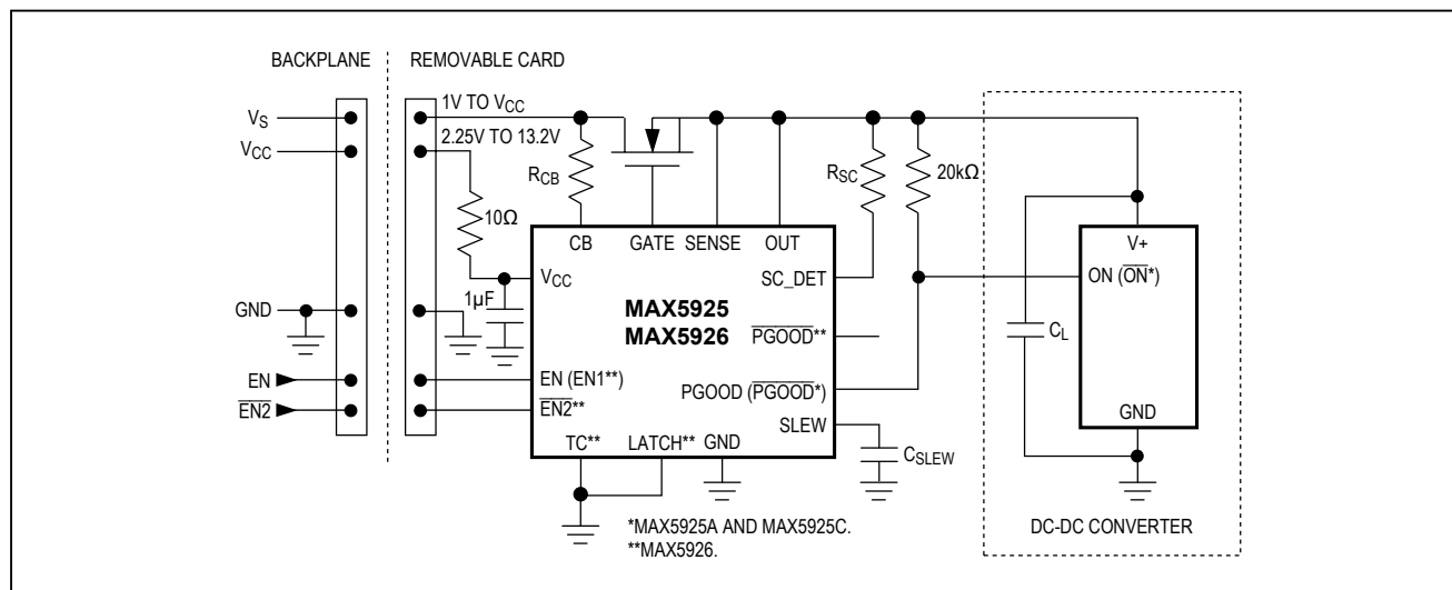
Figure 1. Typical Operating Circuit (Without R_{SENSE} )
