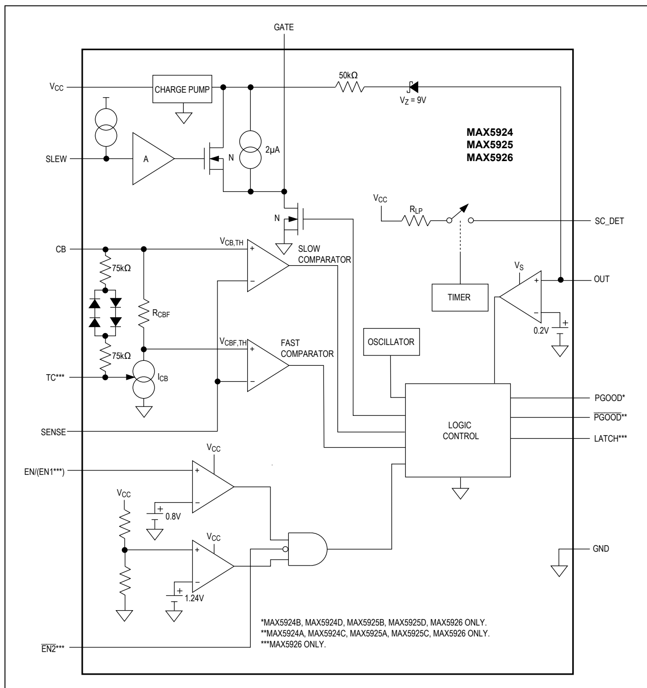
Figure 3. Functional Diagram
