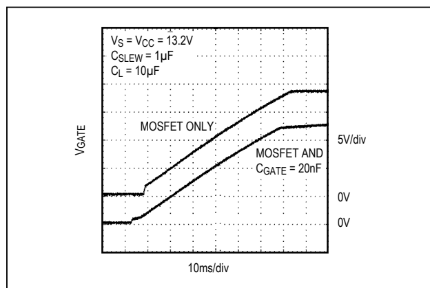
Figure 9. Impact of C_{GATE} on the V_{GATE} Waveform
