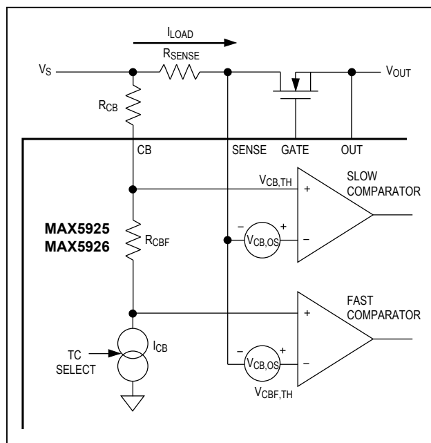
Figure 13. Circuit Breaker Using R_{SENSE}
