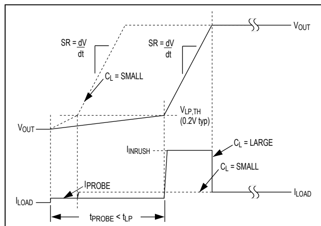
Figure 5. Startup Waveform
