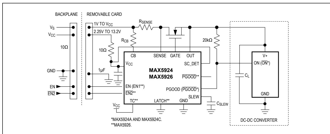
Figure 2. Typical Operating Circuit (With R_{SENSE} )
