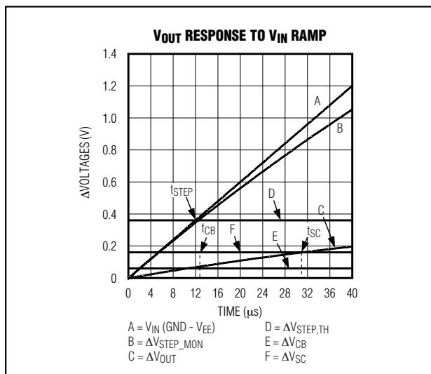
Figure 21. V_{OUT} Response to V_{IN} Ramp of 30V/ms
