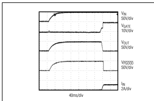
Figure 4. MAX5936 Normal Condition
