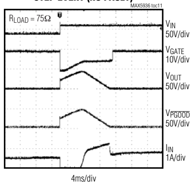
MAX5936_A INPUT VOLTAGE STEP EVENT (NO FAULT)
