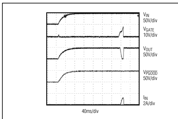
Figure 5. MAX5936 Startup in Fault Condition
