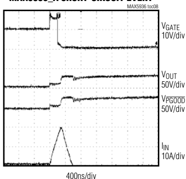
MAX5936_A SHORT-CIRCUIT EVENT
