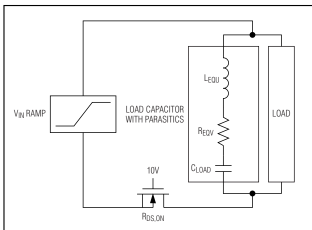
Figure 18. V_{IN} Ramp Test of Load
