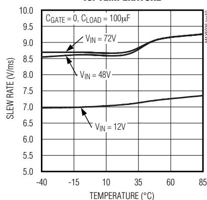
V_{OUT} SLEW RATE vs. TEMPERATURE
