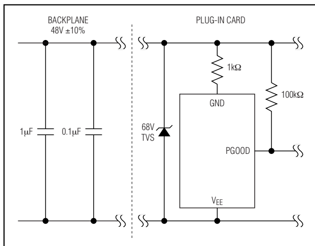
Figure 17. Protecting the MAX5936/MAX5937 Input from High-Voltage Transients
