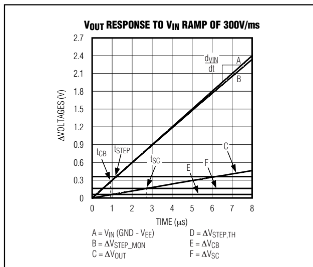
Figure 20. V_{OUT} Response to V_{IN} Ramp of 300V/ms
