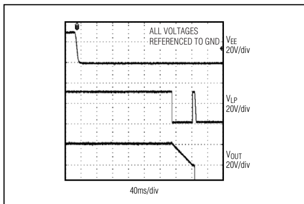
Figure 3. Load Probe Test During Initial Power-Up
