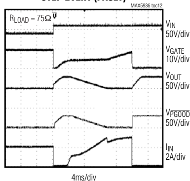
MAX5936_A INPUT VOLTAGE STEP EVENT (FAULT)
