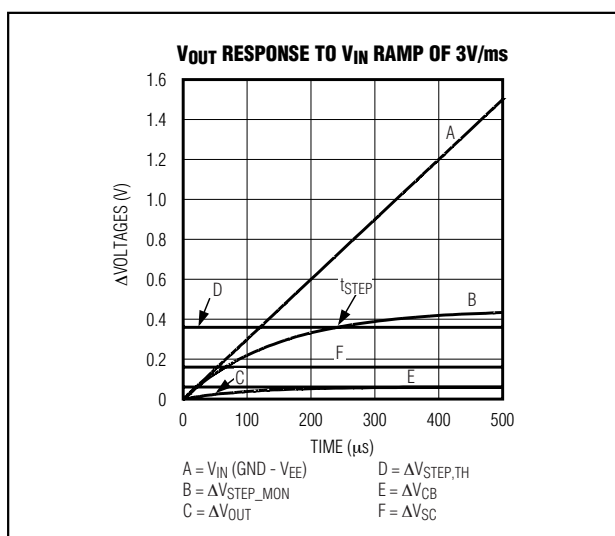
Figure 22. V_{OUT} Response to V_{IN} Ramp of 3V/ms
