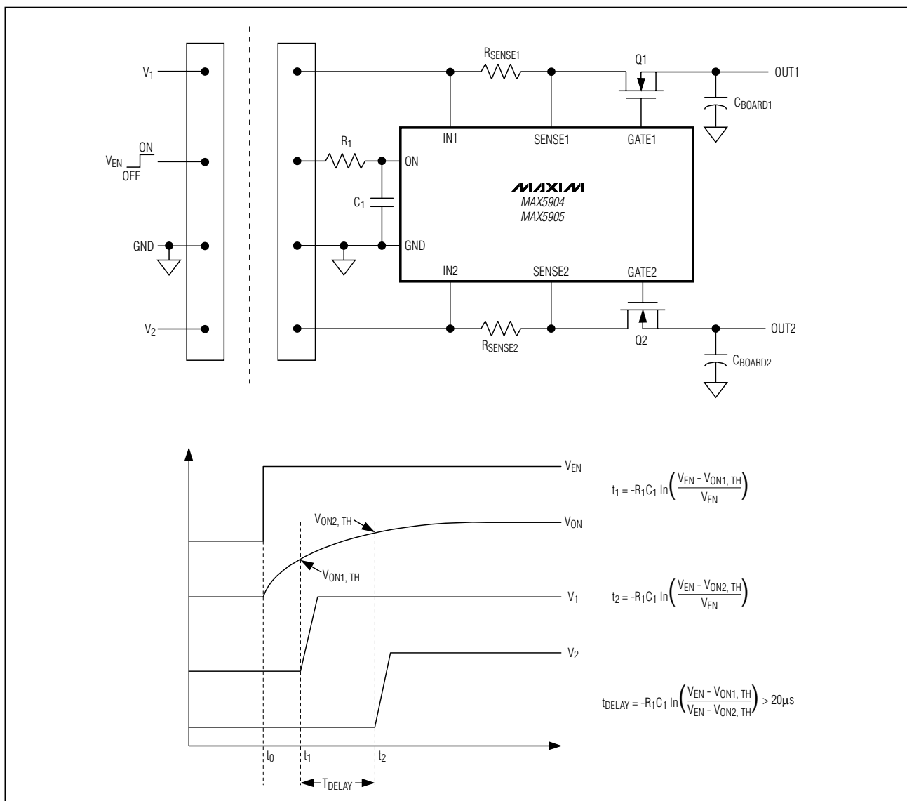
Figure 11. Power Sequencing: Channel 2 Turns On t_{\text{DELAY}} After Channel 1
