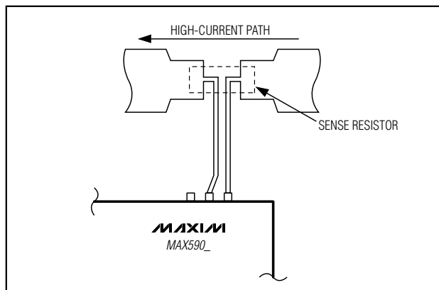
Figure 14. Kelvin Connection for the Current-Sense Resistors
