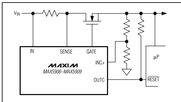
Figure 12. Power-On Reset
