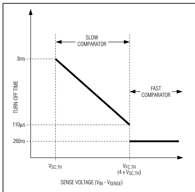
Figure 9. VariableSpeed/BiLevel Response
