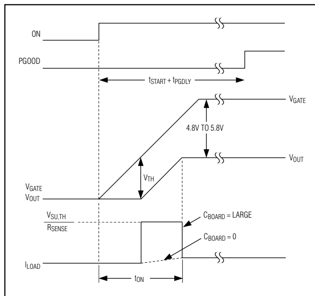
Figure 2. Startup Waveforms
