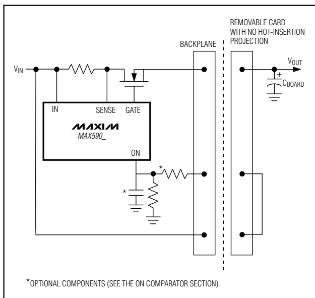
Figure 13. Using the MAX5904-MAX5909 on a Backplane
