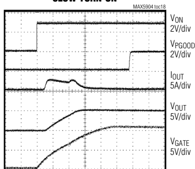
STARTUP WAVEFORMS SLOW TURN-ON
