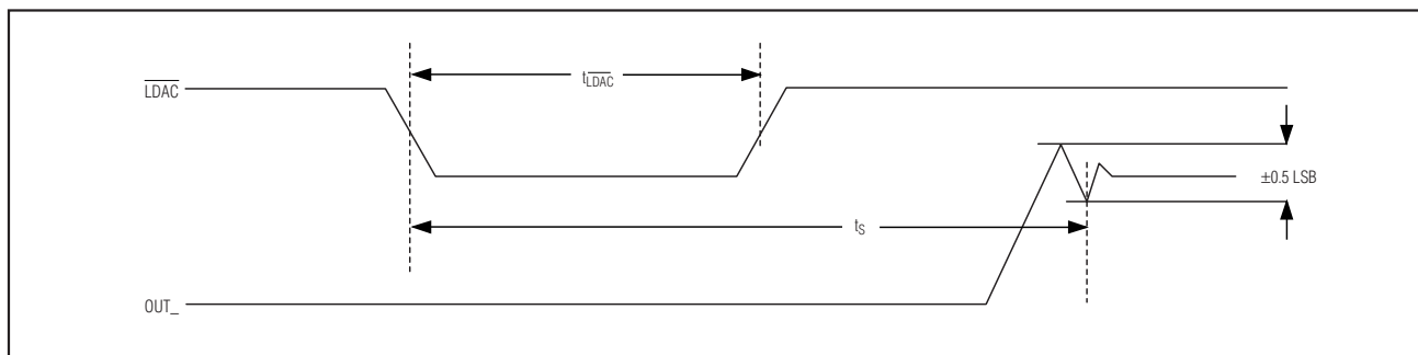
Figure 2. LDAC Timing
