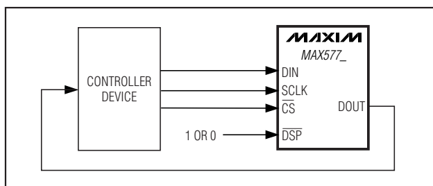
Figure 8. Stand-Alone Configuration
