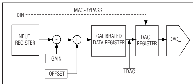
Figure 4. MAC-Bypass Functional Diagram
