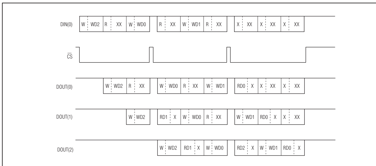
Figure 7. Example 2 of a Daisy-Chain Data Sequence
