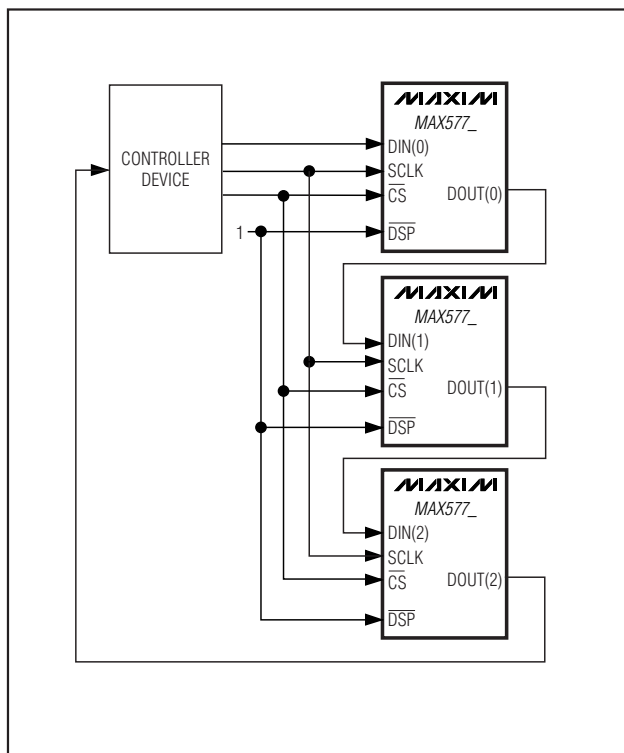
Figure 5. Daisy-Chain Configuration
