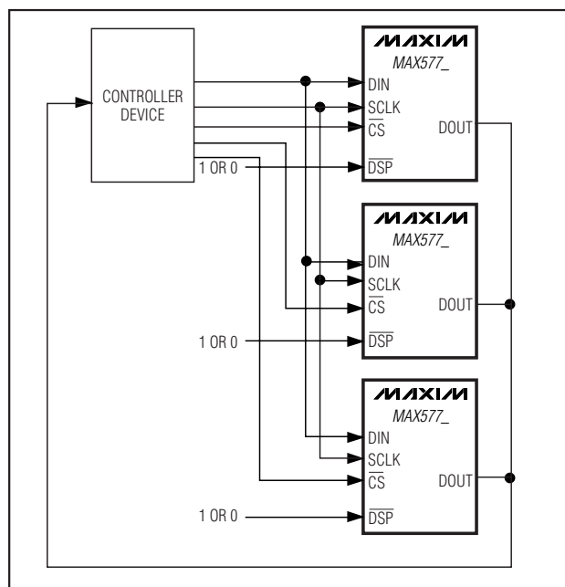
Figure 9. Example of a Parallel Configuration with Readback
