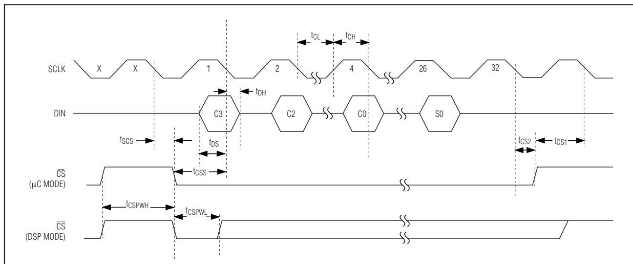
Figure 1. Serial-Interface Timing
