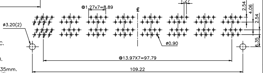
PC Board Layout Component Side Shown Thickness=1.6mm
