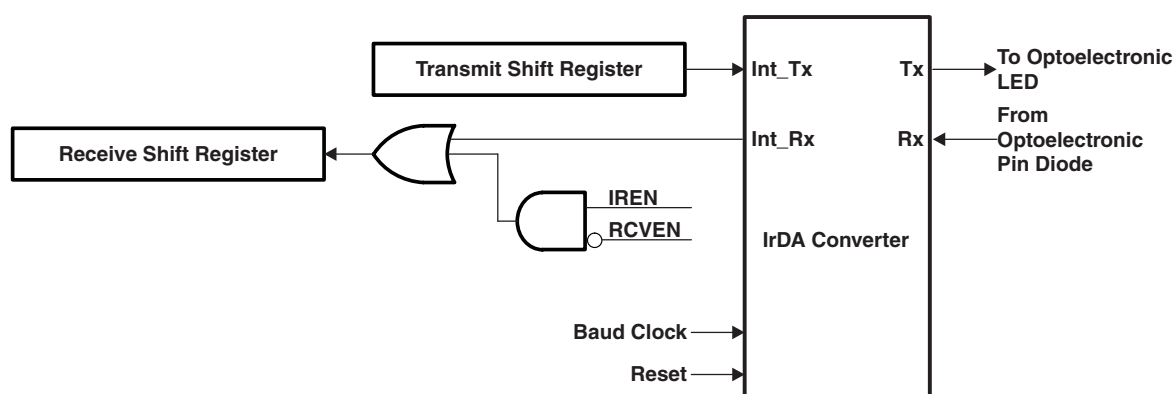
Figure 26. IrDA Mode
