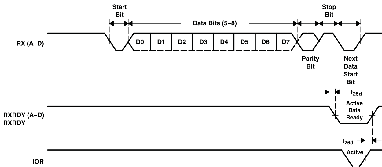
Figure 17. Receive Ready Timing in Non-FIFO Mode
