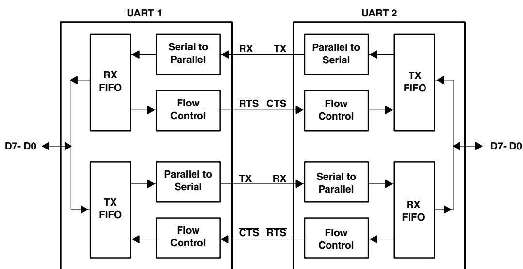
Figure 3. Autoflow Control (Auto-RTS and Auto-CTS) Example
