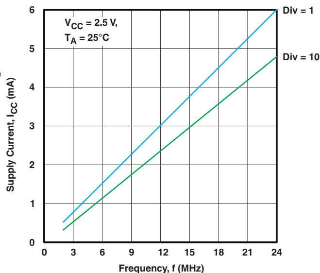
Figure 10. Supply Current vs Frequency (V CC = 2.5 V)
