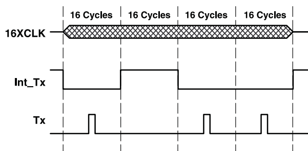
Figure 28. Encoding Scheme – Macro View
