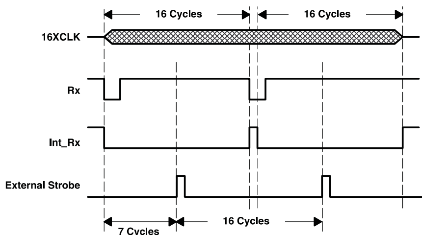
Figure 32. Recommended Strobing For Decoded Data
