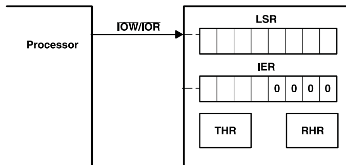
Figure 6. FIFO Polled Mode Operation
