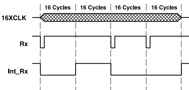
Figure 30. IrDA-SIR Decoding Scheme – Macro View
