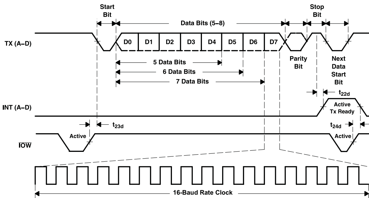
Figure 19. Transmit Timing
