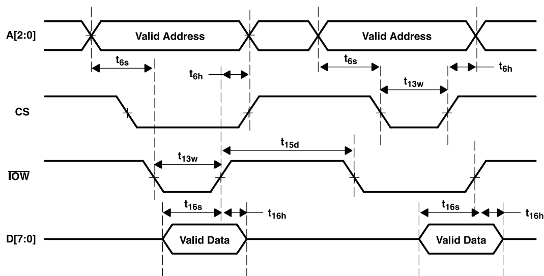
Figure 13. General Write Timing
