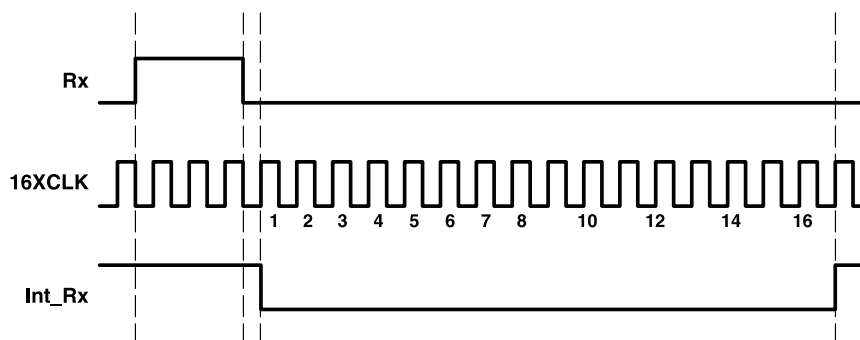
Figure 33. Positive Rx Pulse Decode – Detailed View
