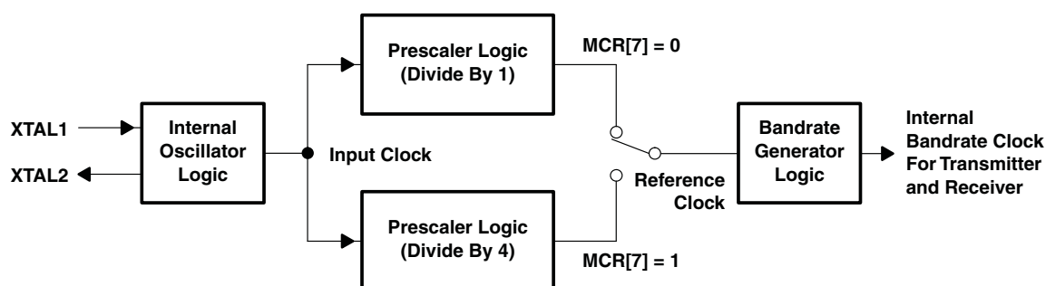
Figure 7. Prescaler and Baud Rate Generator Block Diagram
