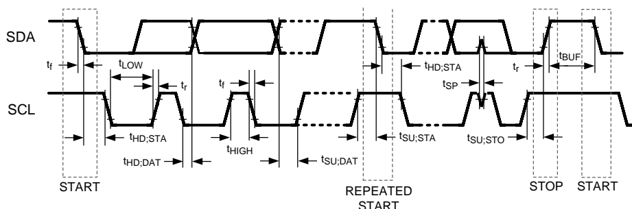
Figure 4. Serial Timing Diagram
