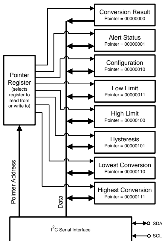
Figure 24. Register Structure
