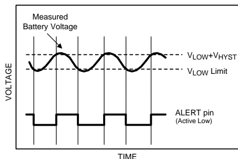
Figure 41. Trickle Charge
