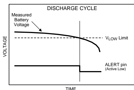
Figure 40. Discharge Cycle
