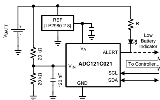
Figure 38. Intelligent Battery Monitor Circuit
