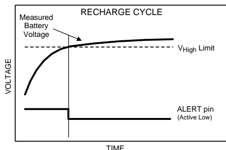
Figure 39. Recharge Cycle
