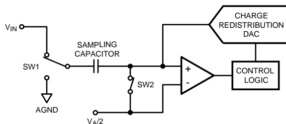
Figure 20. ADC121C021 in Track Mode
