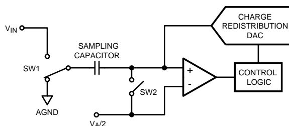
Figure 21. ADC121C021 in Hold Mode
