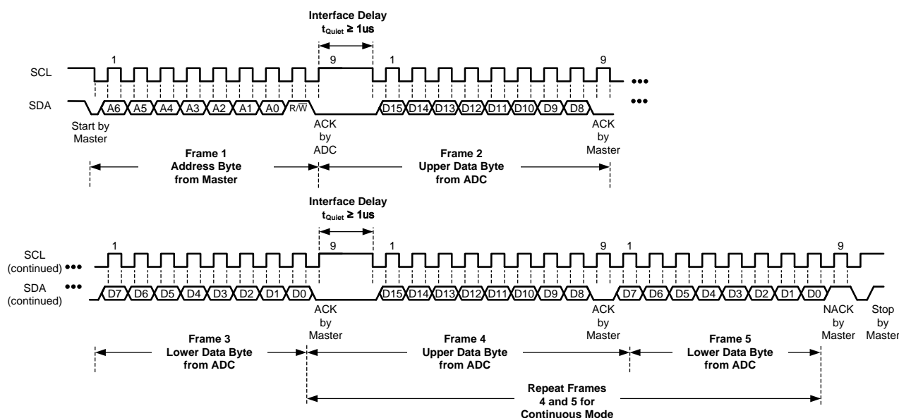
Figure 35. Reading in Quiet Interface Mode
