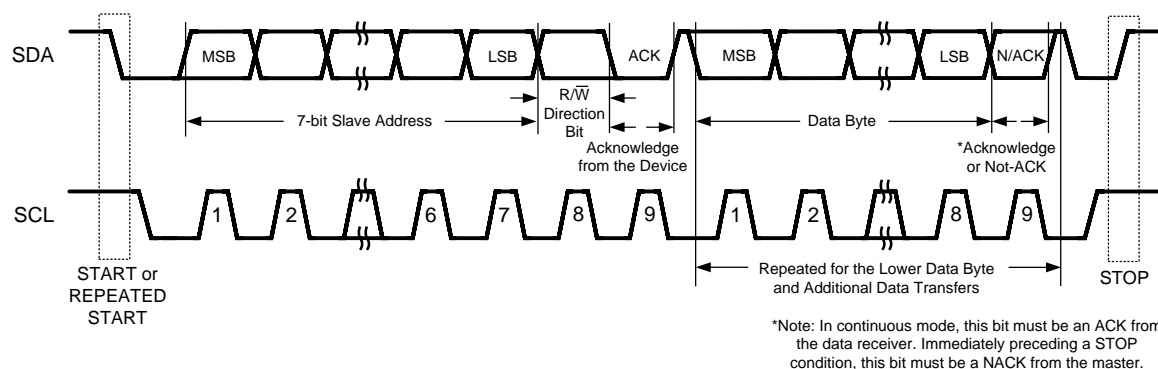
Figure 25. Basic Operation.
