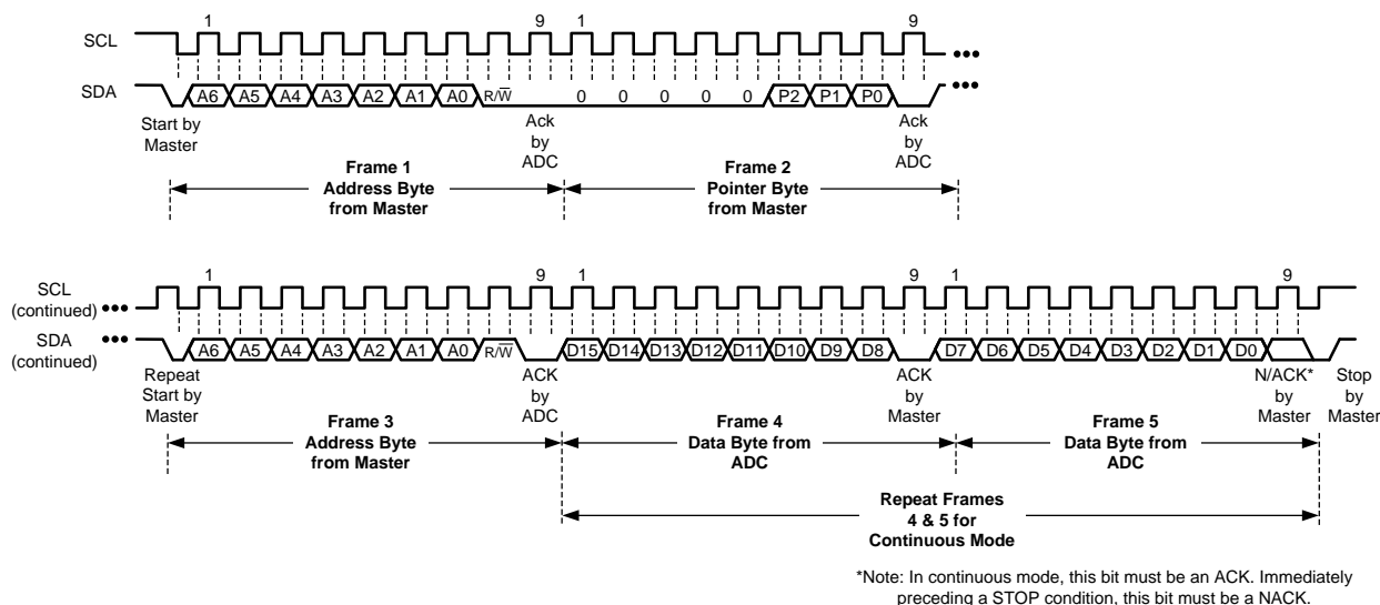
Figure 30. (b) Typical Pointer Set Followed by Immediate Read of a 2-Byte ADC Register
