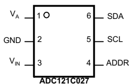
Figure 2. 6-Pin SOT See DDC Package
