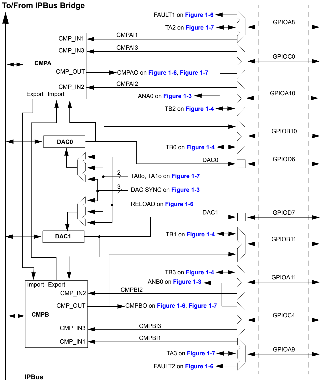
Figure 1-5 56F8037/56F8027 I/O Pin-Out Muxing (Part 3/5)
