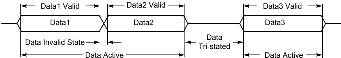
Figure 10-3 Signal States
