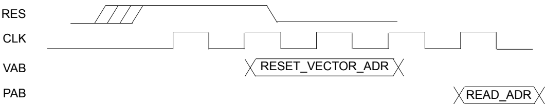
Figure 5-22 Reset Interface
