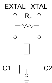
Figure 3-2 External Ceramic Resonator Circuit
