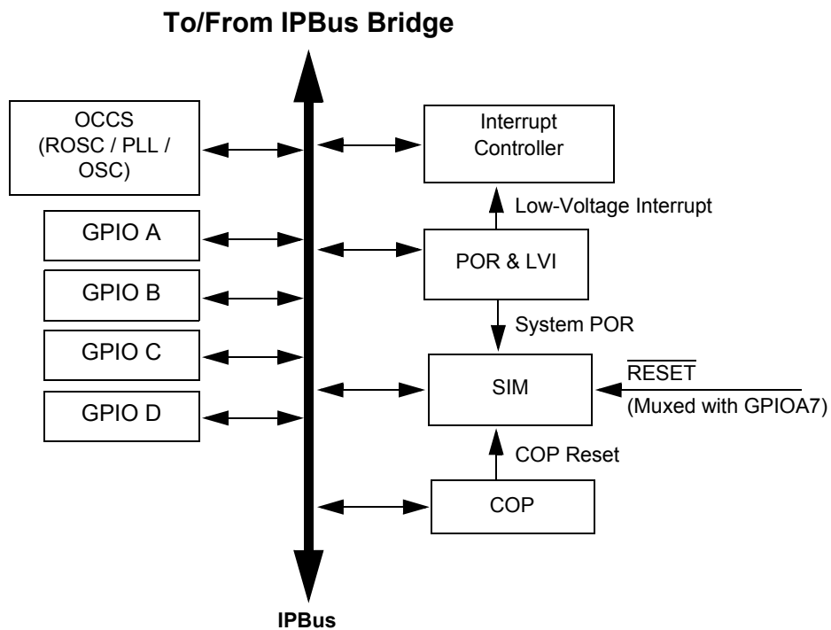
Figure 1-2 Peripheral Subsystem
