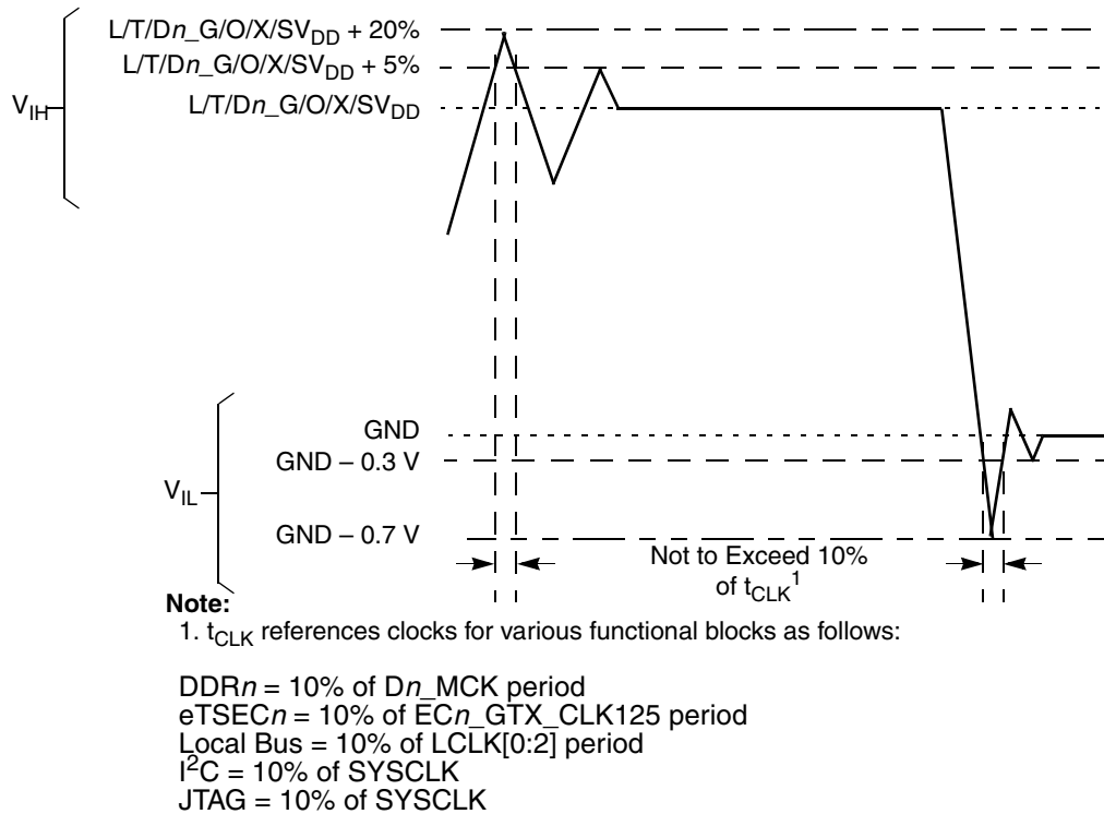
Figure 2. Overshoot/Undershoot Voltage for Dn_M/O/L/TV IN
