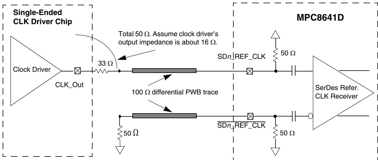
Figure 46. Single-Ended Connection (Reference Only)
