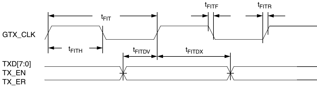
Figure 8. FIFO Transmit AC Timing Diagram
