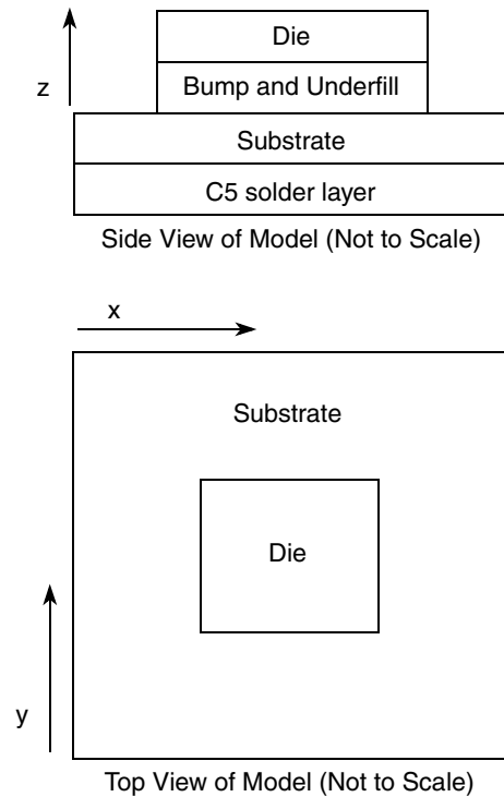
Figure 62. Recommended Thermal Model of MPC8641
