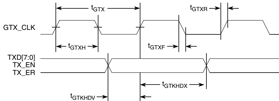
Figure 10. GMII Transmit AC Timing Diagram
