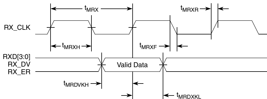
Figure 15. MII Receive AC Timing Diagram
