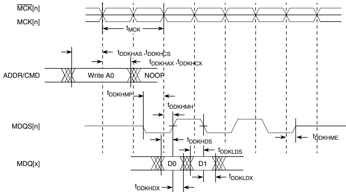
Figure 6. DDR SDRAM Output Timing Diagram
