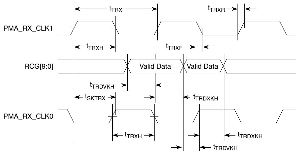
Figure 17. TBI Receive AC Timing Diagram
