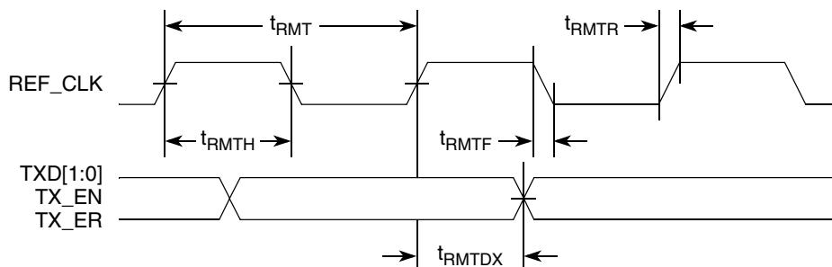
Figure 20. RMII Transmit AC Timing Diagram
