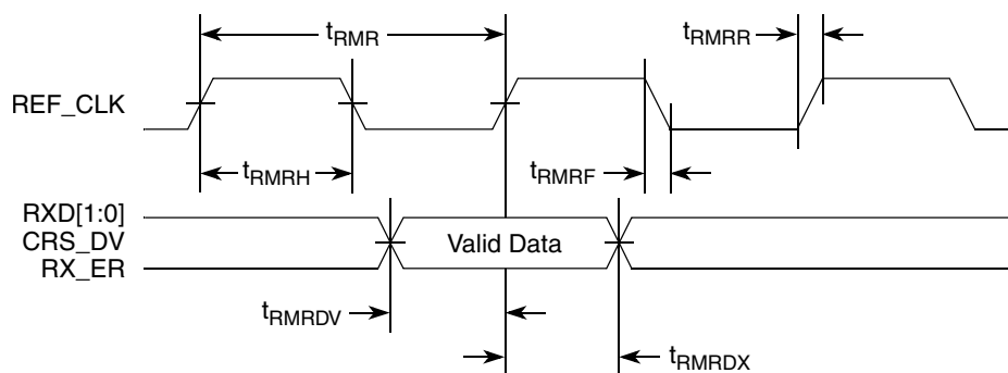
Figure 22. RMII Receive AC Timing Diagram
