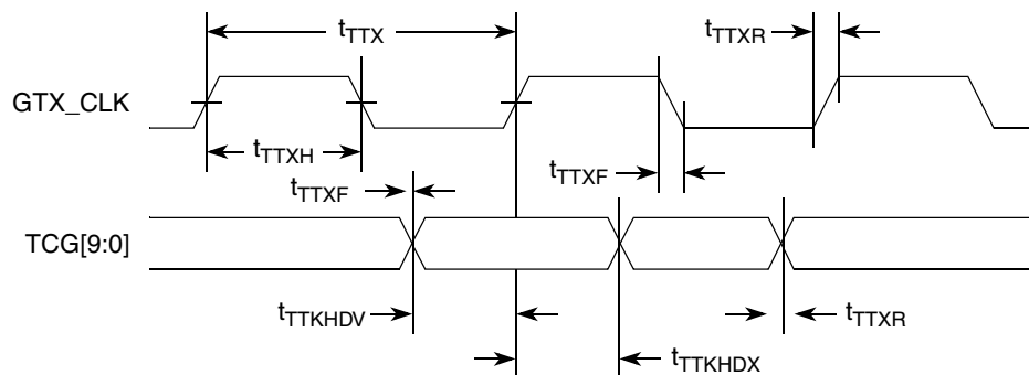
Figure 16. TBI Transmit AC Timing Diagram
