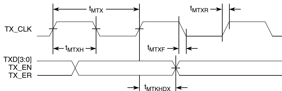
Figure 13. MII Transmit AC Timing Diagram
