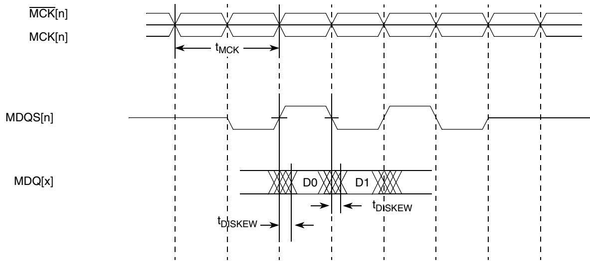
Figure 4. DDR Input Timing Diagram for t_{DISKEW}
