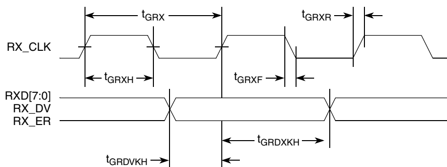
Figure 12. GMII Receive AC Timing Diagram
