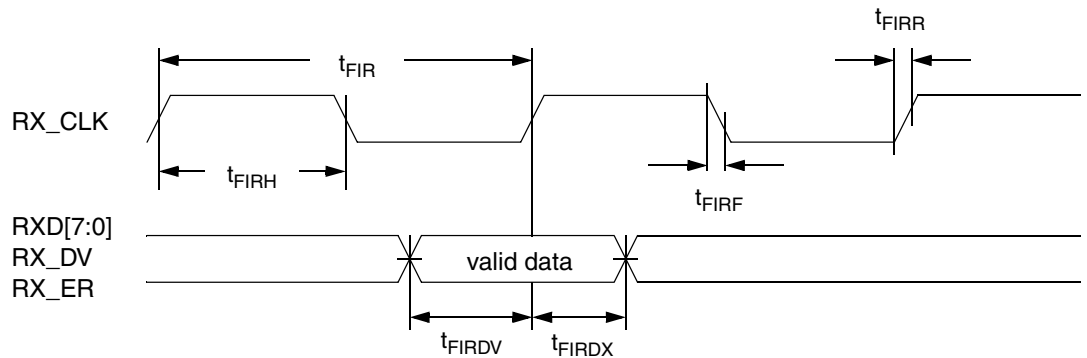
Figure 9. FIFO Receive AC Timing Diagram
