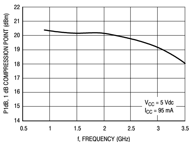
Figure 5. P1dB versus Frequency
