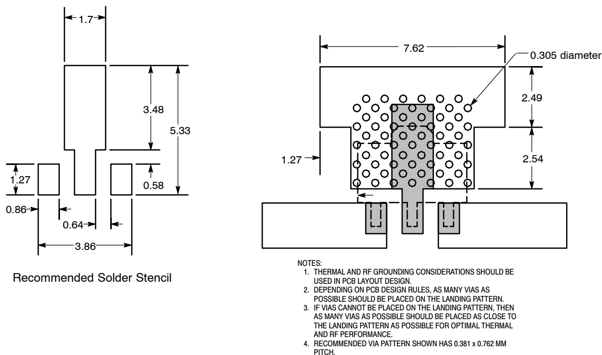
Figure 20. Recommended Mounting Configuration
