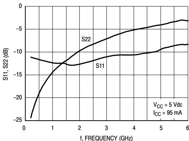
Figure 3. Input/Output Loss versus Frequency
