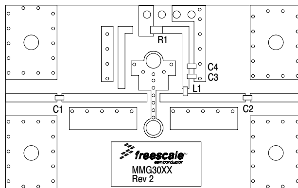
Figure 19. 50 Ohm Test Circuit Component Layout
