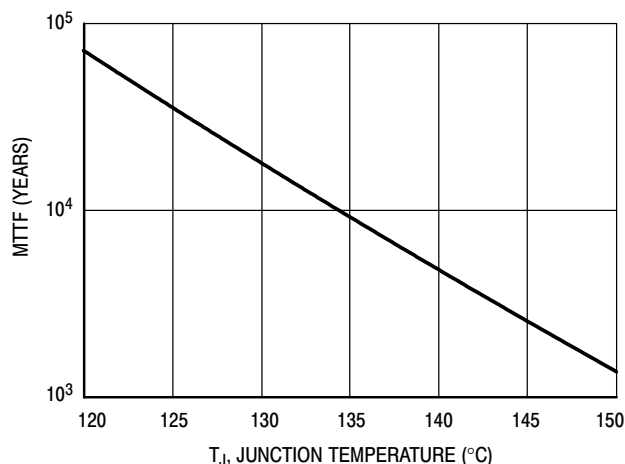
Figure 11. MTTF versus Junction Temperature
