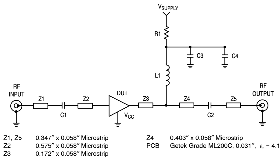
Figure 17. 50 Ohm Test Circuit Schematic
