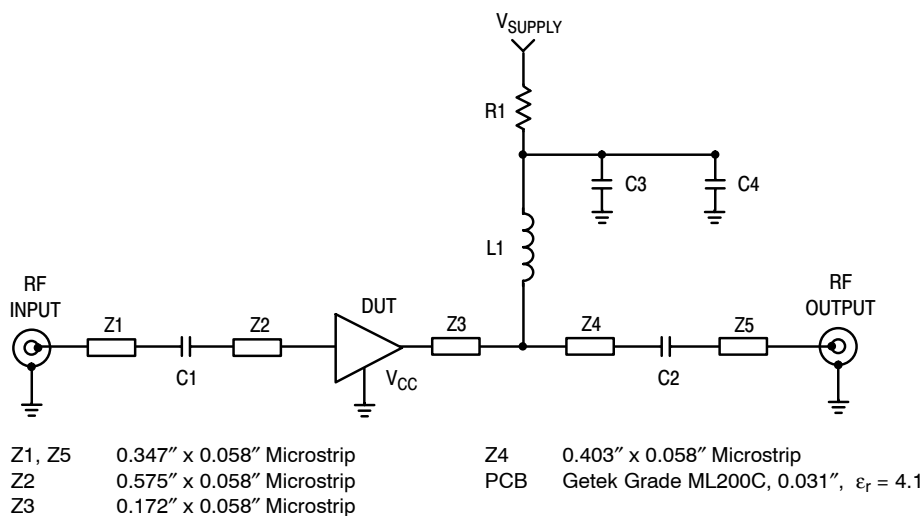
Figure 14. 50 Ohm Test Circuit Schematic
