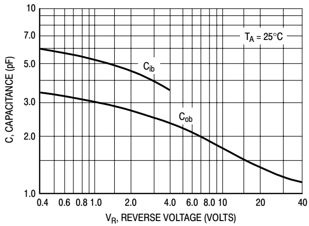
Figure 5. Capacitances
