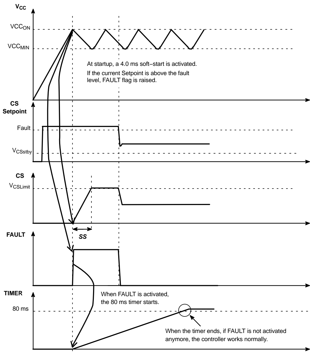
Figure 3. Startup Sequence
