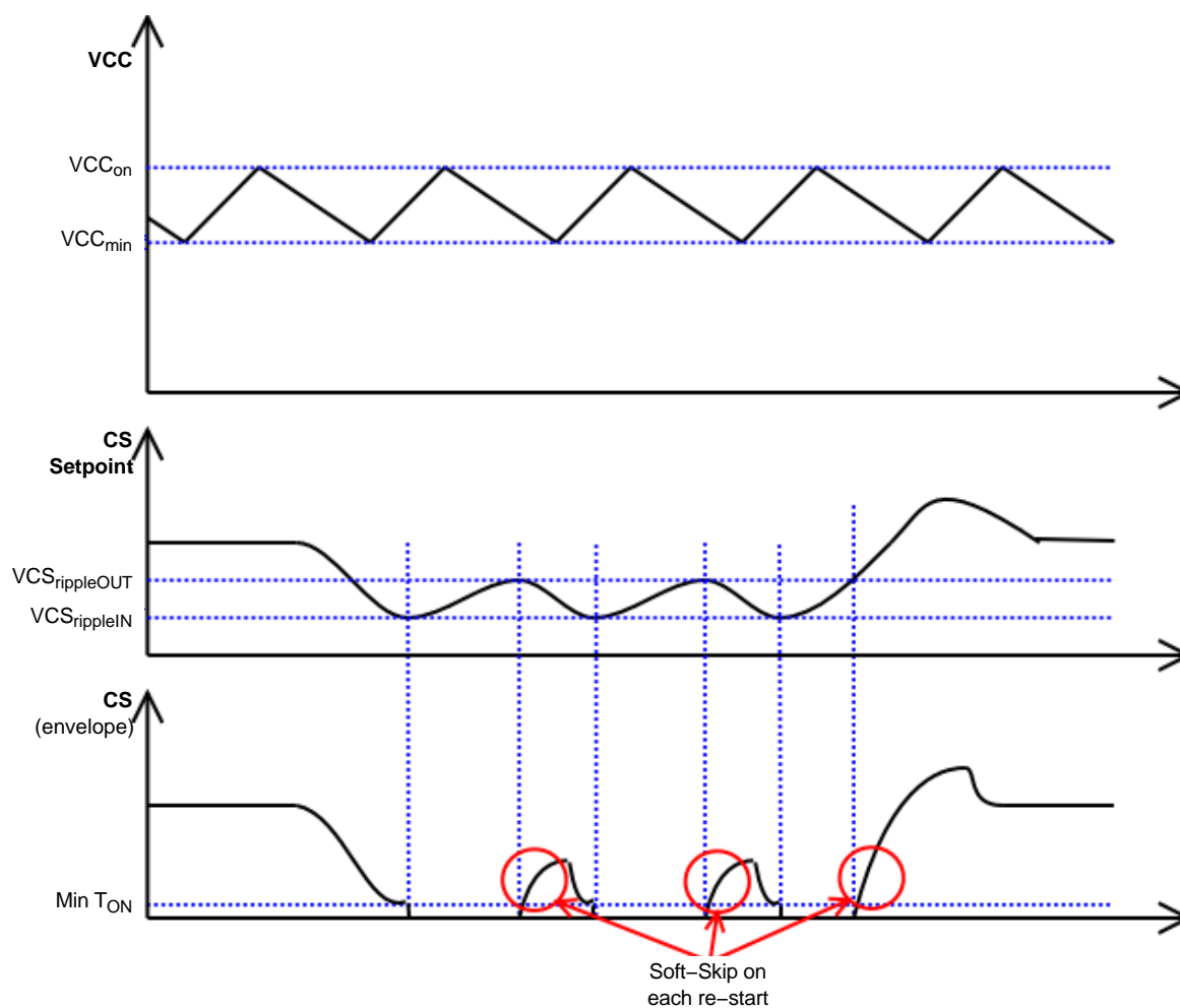
Figure 5. Soft-Skip Mode in Standby
