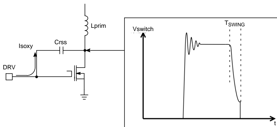
Figure 6. Soxyless Concept
