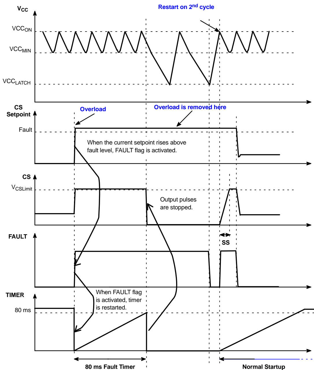
Figure 4. Overload
