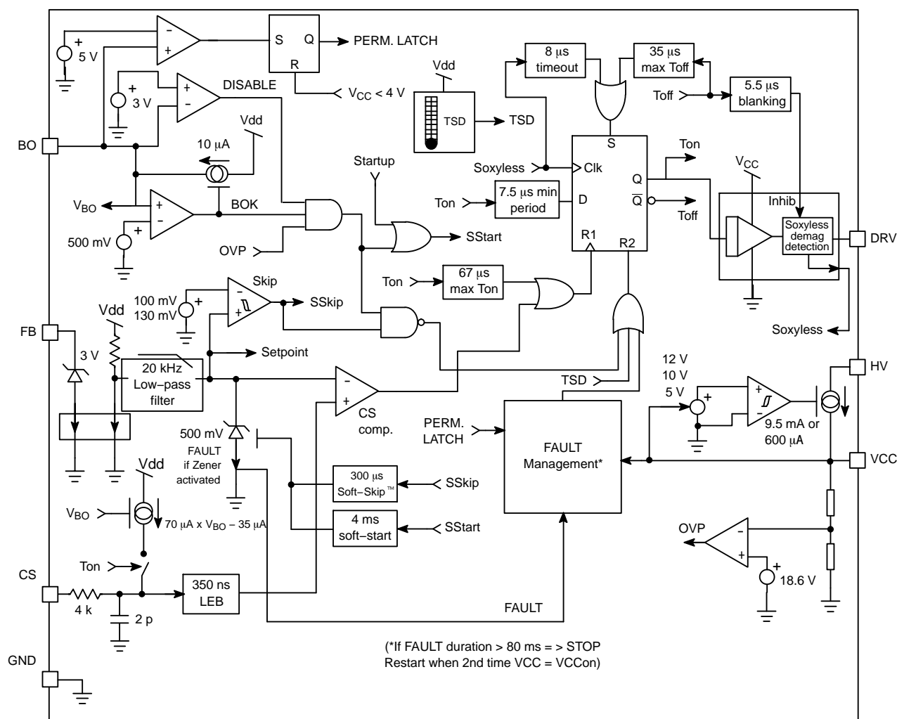
Figure 2. Internal Circuit Architecture
