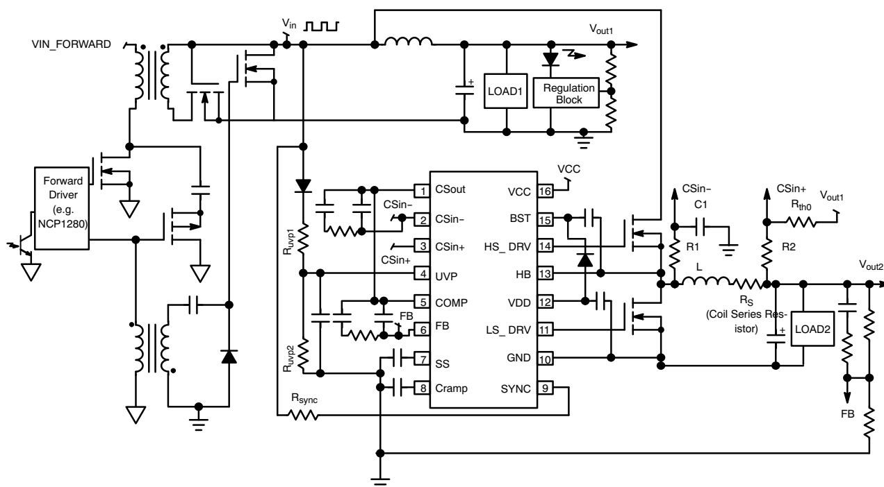
Figure 27. Post-Regulation with CCCV Protection
