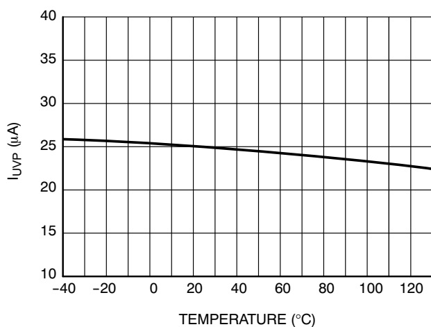
Figure 15. UVP Current Source versus Temperature
