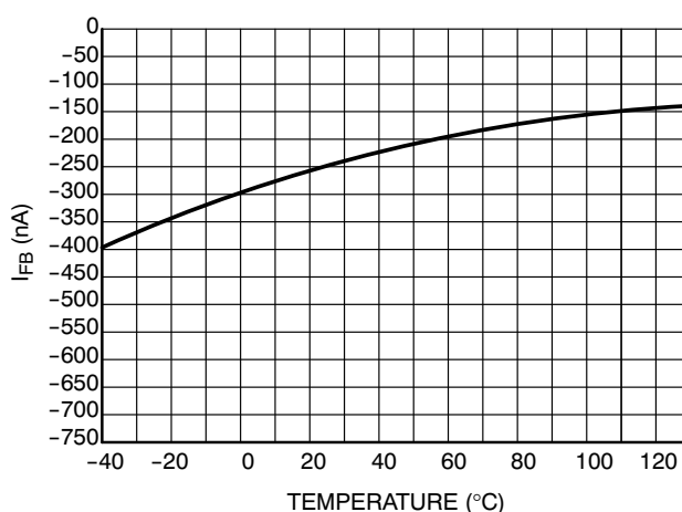
Figure 4. FB Pin Bias Current versus Temperature
