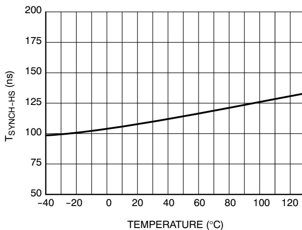
Figure 16. Delay Synchronization Pulse to HS High versus Temperature
