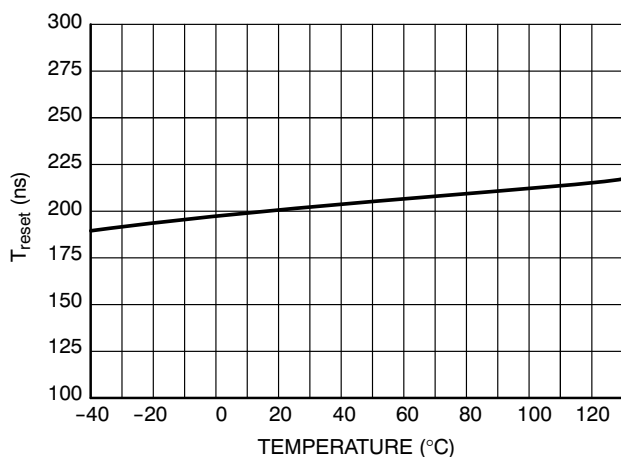
Figure 17. Reset Time versus Temperature
