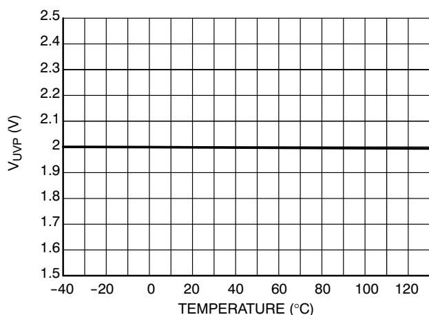
Figure 13. UVP Threshold versus Temperature
