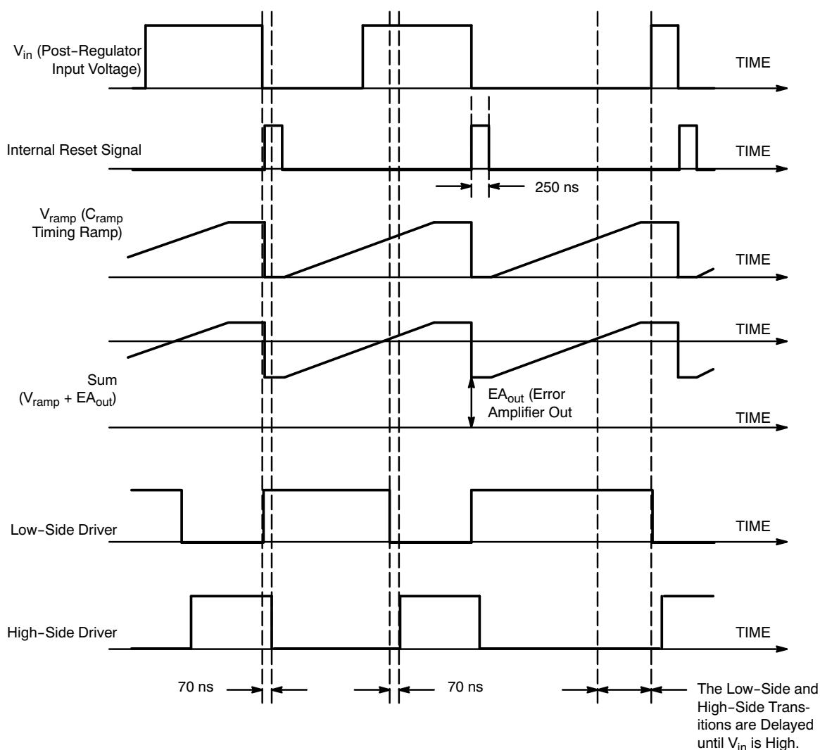
Figure 22. Timing Diagram
