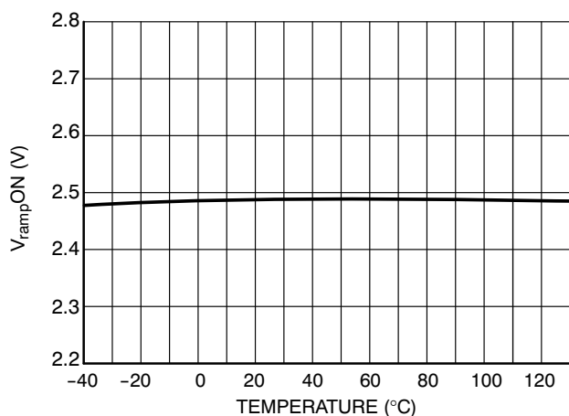
Figure 9. V rampON versus Temperature @ V pin5 = 0.5 V
