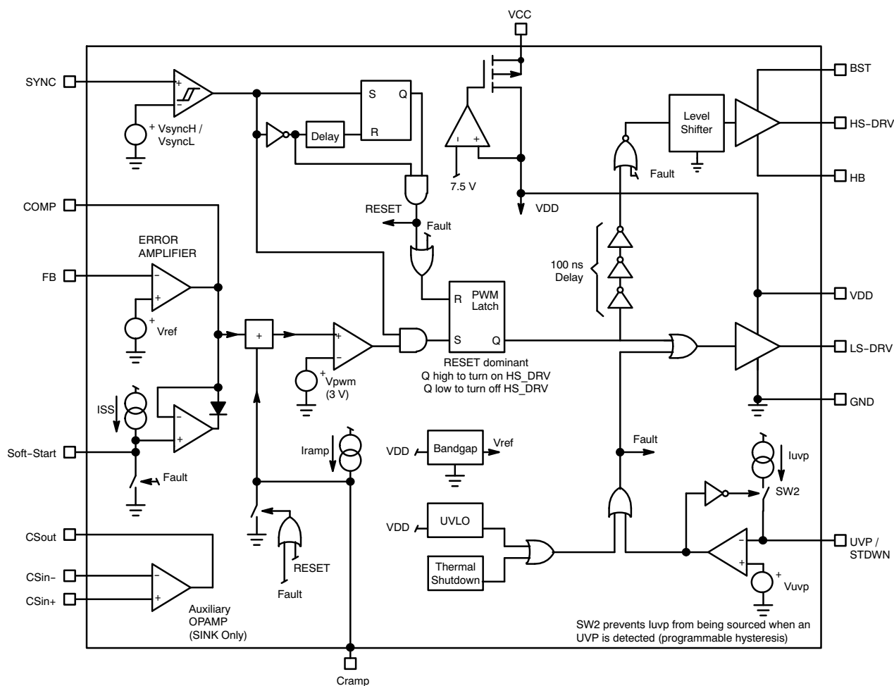
Figure 2. Block Diagram
