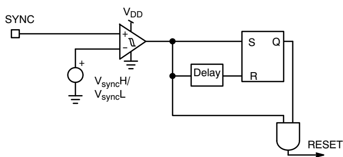
Figure 24. Synchronization Block
