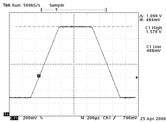
Figure 12. 1.6 to 0.5 Dynamic VID Response
