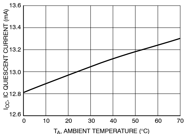
Figure 5. IC Quiescent Current vs. Ambient Temperature
